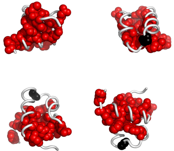
Fig. 3. Residues in IguuA, colored according to the cluster they belong to: red, followed by blue and yellow are the largest clusters (see Appendix for the coloring scheme). Clockwise: front, back, top and bottom views. The corresponding Pymol script is attached.
