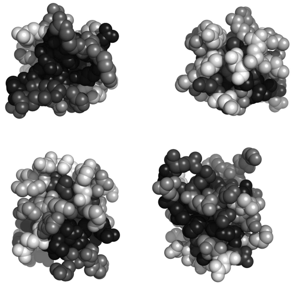
Fig. 2. Residues in IguuA, colored by their relative importance. Clockwise: front, back, top and bottom views.
