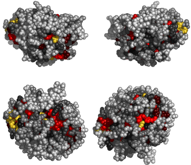
Fig. 3. Residues in IgvoA, colored by their relative importance. Clockwise: front, back, top and bottom views.
