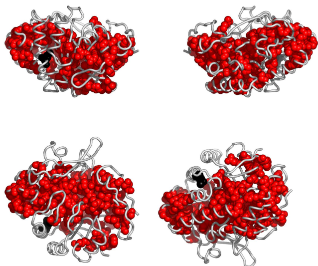
Fig. 4. Residues in 1gvoA, colored according to the cluster they belong to: red, followed by blue and yellow are the largest clusters (see Appendix for the coloring scheme). Clockwise: front, back, top and bottom views. The corresponding Pymol script is attached.
