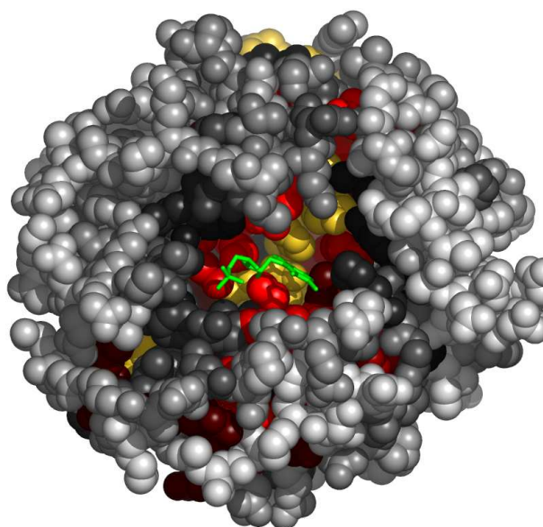
Fig. 6. Residues in IgvoA, at the interface with FMN, colored by their relative importance. The ligand (FMN) is colored green. Atoms further than 30Å away from the geometric center of the ligand, as well as on the line of sight to the ligand were removed. (See Appendix for the coloring scheme for the protein chain IgvoA.)
