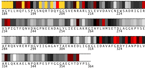
Fig. 2. Residues 184-364 in IgvoA colored by their relative importance. (See Appendix, Fig.9, for the coloring scheme.)
