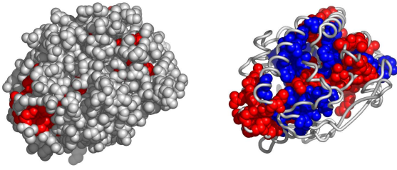
Fig. 8. Another possible active surface on the chain 1gvoA. The larger cluster it belongs to is shown in blue.
