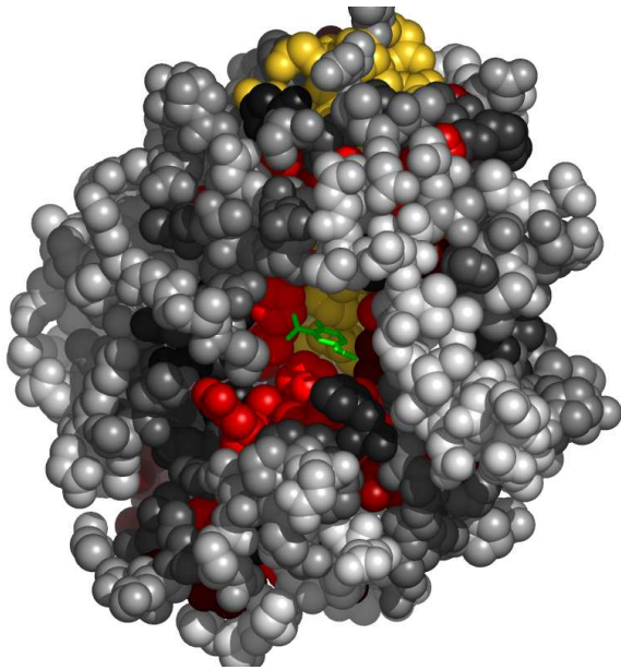
Fig. 5. Residues in 1gvoA, at the interface with 2,4-dinitrophenol, colored by their relative importance. The ligand (2,4-dinitrophenol) is colored green. Atoms further than 30Å away from the geometric center of the ligand, as well as on the line of sight to the ligand were removed. (See Appendix for the coloring scheme for the protein chain 1gvoA.)
