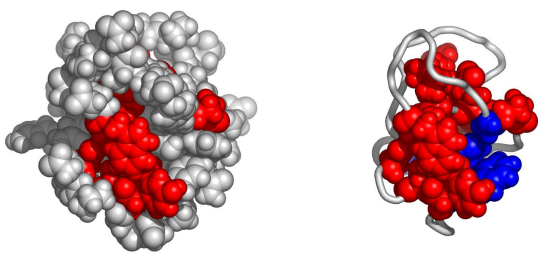
Fig. 4. A possible active surface on the chain 1gyfA. The larger cluster it belongs to is shown in blue.
