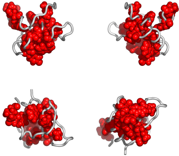
Fig. 3. Residues in 1gyfA, colored according to the cluster they belong to: red, followed by blue and yellow are the largest clusters (see Appendix for the coloring scheme). Clockwise: front, back, top and bottom views. The corresponding Pymol script is attached.
