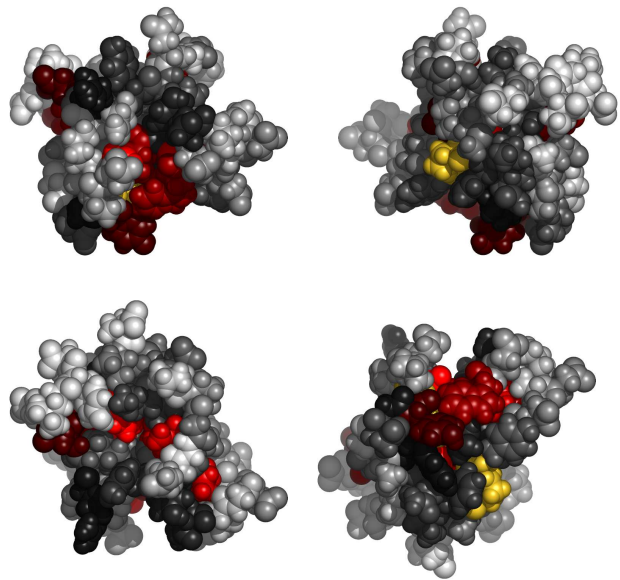
Fig. 2. Residues in 1gyfA, colored by their relative importance. Clockwise: front, back, top and bottom views.
