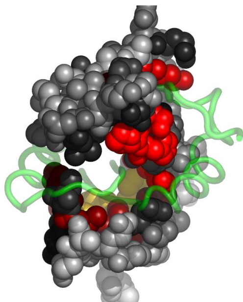
Fig. 4. Residues in 1gyjA, at the interface with 1gyjB, colored by their relative importance. 1gyjB is shown in backbone representation (See Appendix for the coloring scheme for the protein chain 1gyjA.)
