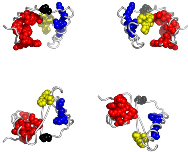
Fig. 3. Residues in 1gyjA, colored according to the cluster they belong to: red, followed by blue and yellow are the largest clusters (see Appendix for the coloring scheme). Clockwise: front, back, top and bottom views. The corresponding Pymol script is attached.
