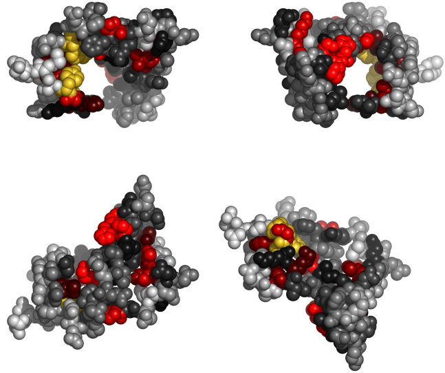
Fig. 2. Residues in 1gyjA, colored by their relative importance. Clockwise: front, back, top and bottom views.
