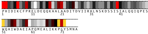
Fig. 1. Residues 1-76 in 1gyjA colored by their relative importance. (See Appendix, Fig.5, for the coloring scheme.)
