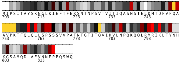
Fig. 1. Residues 703-822 in 1gyuA colored by their relative importance. (See Appendix, Fig.5, for the coloring scheme.)
