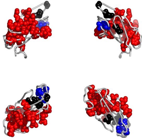
Fig. 2. Residues in 1gyuA, colored by their relative importance. Clockwise: front, back, top and bottom views.
