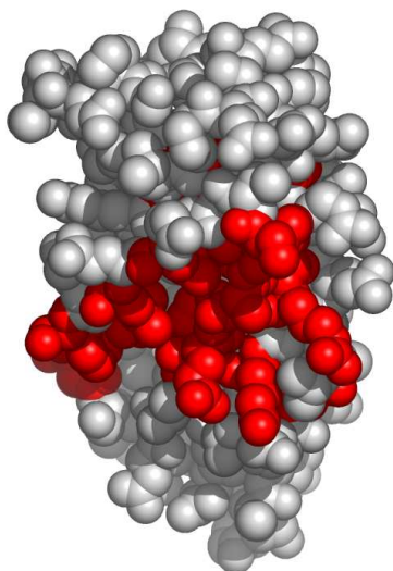
Fig. 4. A possible active surface on the chain IgyuA.
