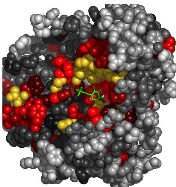
Fig. 7. Residues in 1h0cA, at the interface with PLP, colored by their relative importance. The ligand (PLP) is colored green. Atoms further than 30 Å away from the geometric center of the ligand, as well as on the line of sight to the ligand were removed. (See Appendix for the coloring scheme for the protein chain 1h0cA.)
