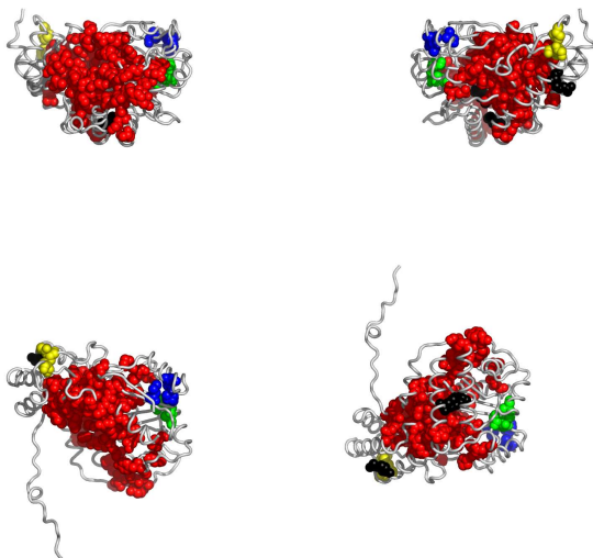
Fig. 4. Residues in 1h0cA, colored according to the cluster they belong to: red, followed by blue and yellow are the largest clusters (see Appendix for the coloring scheme). Clockwise: front, back, top and bottom views. The corresponding Pymol script is attached.
