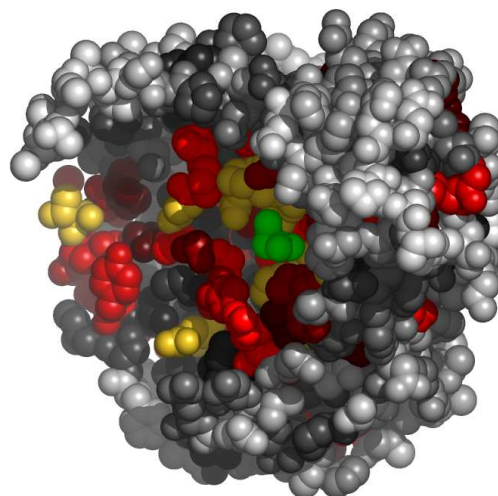
Fig. 6. Residues in 1h0cA, at the interface with AOA, colored by their relative importance. The ligand (AOA) is colored green. Atoms further than 30Å away from the geometric center of the ligand, as well as on the line of sight to the ligand were removed. (See Appendix for the coloring scheme for the protein chain 1h0cA.)
