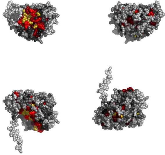
Fig. 3. Residues in 1h0cA, colored by their relative importance. Clockwise: front, back, top and bottom views.
