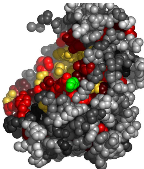
Fig. 8. Residues in 1h0cA, at the interface with glycerol, colored by their relative importance. The ligand (glycerol) is colored green. Atoms further than 30Å away from the geometric center of the ligand, as well as on the line of sight to the ligand were removed. (See Appendix for the coloring scheme for the protein chain 1h0cA.)
