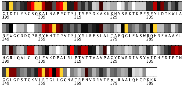
Fig. 2. Residues 199-391 in 1h0cA colored by their relative importance. (See Appendix, Fig.9, for the coloring scheme.)
