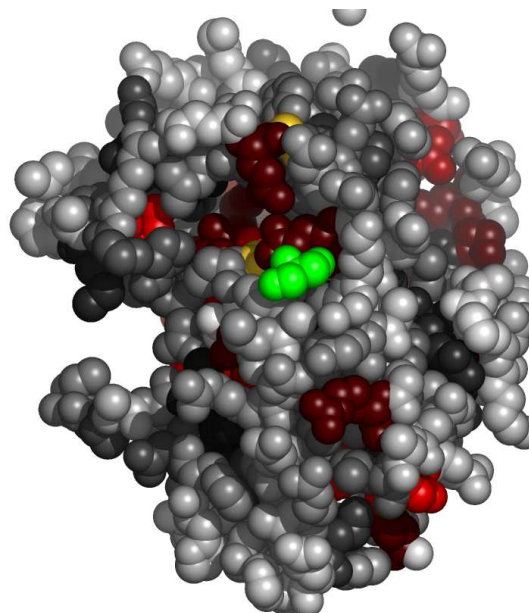
Fig. 5. Residues in 1h0cA, at the interface with glycerol, colored by their relative importance. The ligand (glycerol) is colored green. Atoms further than 30 Å away from the geometric center of the ligand, as well as on the line of sight to the ligand were removed. (See Appendix for the coloring scheme for the protein chain 1h0cA.)
