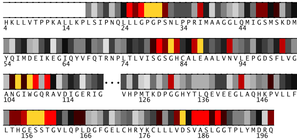
Fig. 1. Residues 4-198 in 1h0cA colored by their relative importance. (See Appendix, Fig.9, for the coloring scheme.)
