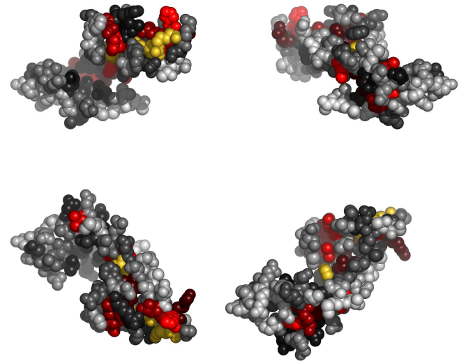
Fig. 1. Residues 55-128 in 1h3oB colored by their relative importance. (See Appendix, Fig.7, for the coloring scheme.)
