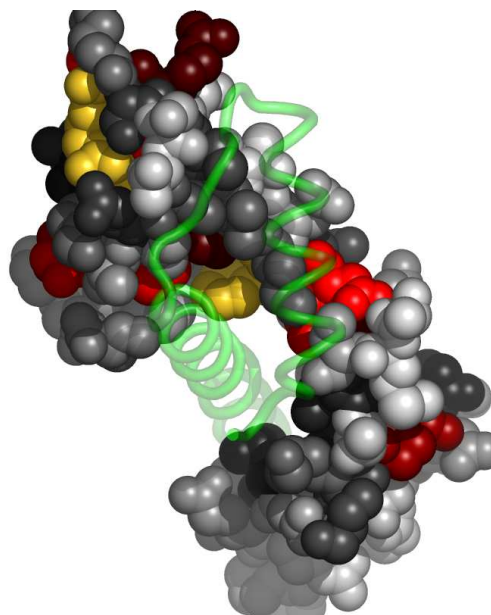
Fig. 4. Residues in 1h3oB, at the interface with 1h3oA, colored by their relative importance. 1h3oA is shown in backbone representation (See Appendix for the coloring scheme for the protein chain 1h3oB.)
