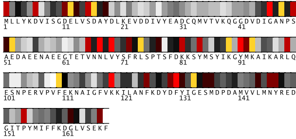
Fig. 1. Residues 1-168 in 1h6qA colored by their relative importance. (See Appendix, Fig.6, for the coloring scheme.)
