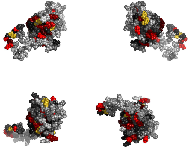
Fig. 1. Residues 1-168 in 1h6qA colored by their relative importance. (See Appendix, Fig.6, for the coloring scheme.)
