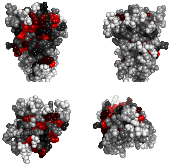
Fig. 2. Residues in 1h7zA, colored by their relative importance. Clockwise: front, back, top and bottom views.
