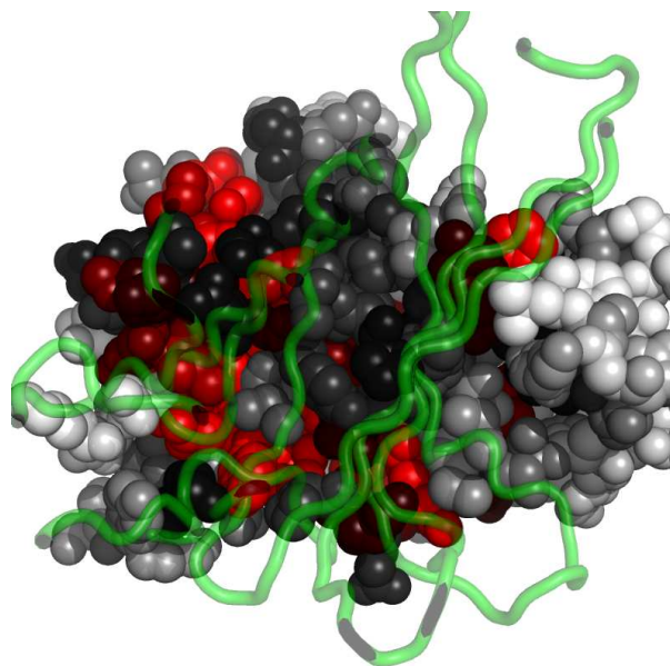
Fig. 5. Residues in 1h7zA, at the interface with 1h7zC, colored by their relative importance. 1h7zC is shown in backbone representation (See Appendix for the coloring scheme for the protein chain 1h7zA.)
