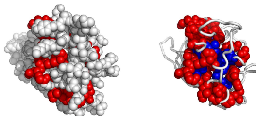
Fig. 6. A possible active surface on the chain 1h7zA. The larger cluster it belongs to is shown in blue.
