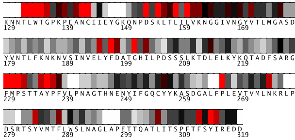
Fig. 1. Residues 129-319 in 1h7zA colored by their relative importance. (See Appendix, Fig.7, for the coloring scheme.)
