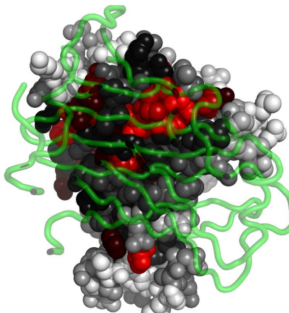
Fig. 4. Residues in 1h7zA, at the interface with 1h7zB, colored by their relative importance. 1h7zB is shown in backbone representation (See Appendix for the coloring scheme for the protein chain 1h7zA.)
