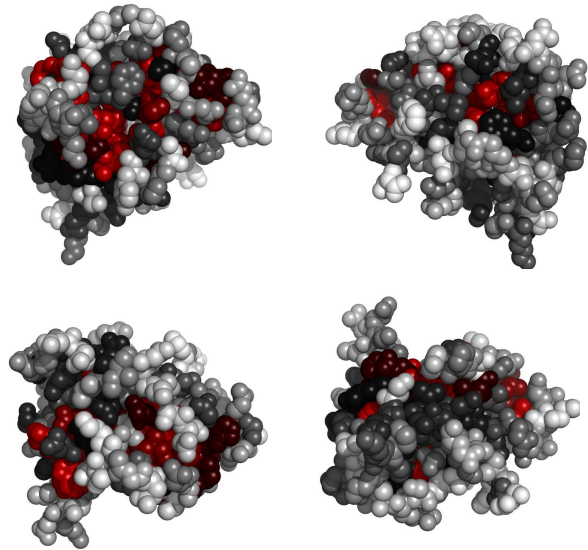
Fig. 2. Residues in IhibA, colored by their relative importance. Clockwise: front, back, top and bottom views.
