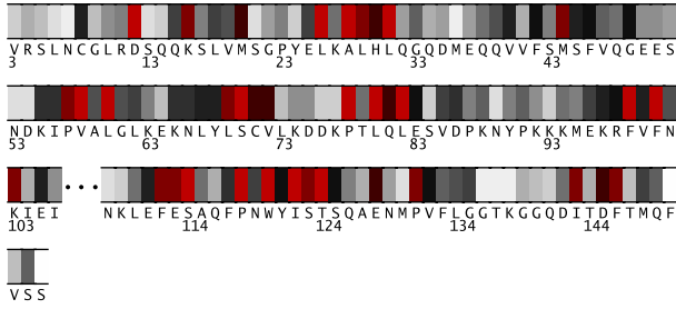
Fig. 1. Residues 3-153 in IhibA colored by their relative importance. (See Appendix, Fig.5, for the coloring scheme.)
