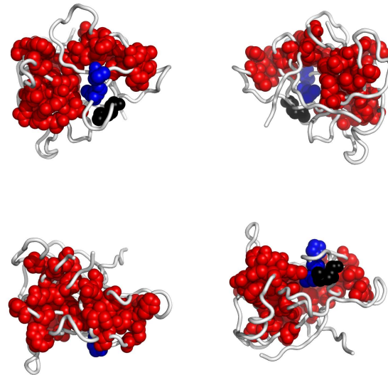
Fig. 3. Residues in IhibA, colored according to the cluster they belong to: red, followed by blue and yellow are the largest clusters (see Appendix for the coloring scheme). Clockwise: front, back, top and bottom views. The corresponding Pymol script is attached.
