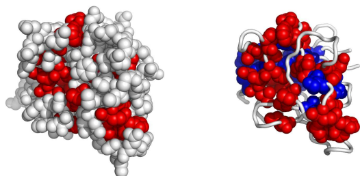
Fig. 4. A possible active surface on the chain 1hibA. The larger cluster it belongs to is shown in blue.
