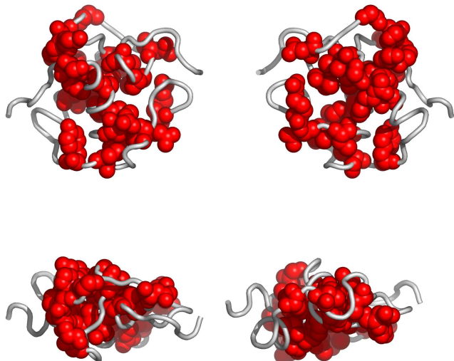
Fig. 2. Residues in IhraA, colored by their relative importance. Clockwise: front, back, top and bottom views.
