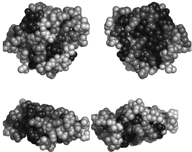
Fig. 1. Residues 1-80 in IhraA colored by their relative importance. (See Appendix, Fig.4, for the coloring scheme.)
