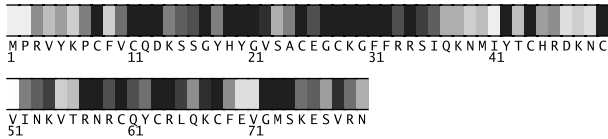
Fig. 1. Residues 1-80 in IhraA colored by their relative importance. (See Appendix, Fig.4, for the coloring scheme.)
