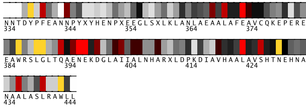
Fig. 1. Residues 334-445 in 1hxiA colored by their relative importance. (See Appendix, Fig.6, for the coloring scheme.)
