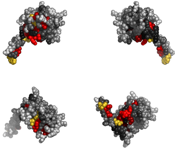
Fig. 2. Residues in 1hxiA, colored by their relative importance. Clockwise: front, back, top and bottom views.
