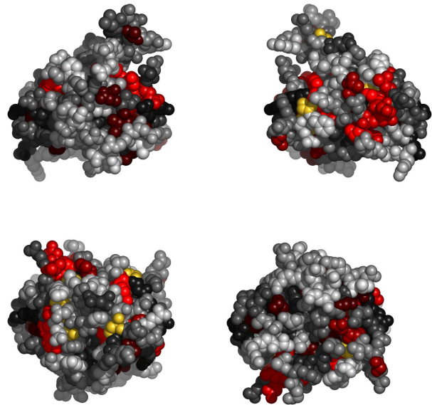
Fig. 2. Residues in li04A, colored by their relative importance. Clockwise: front, back, top and bottom views.
