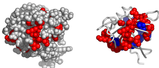
Fig. 4. A possible active surface on the chain 1i04A. The larger cluster it belongs to is shown in blue.
