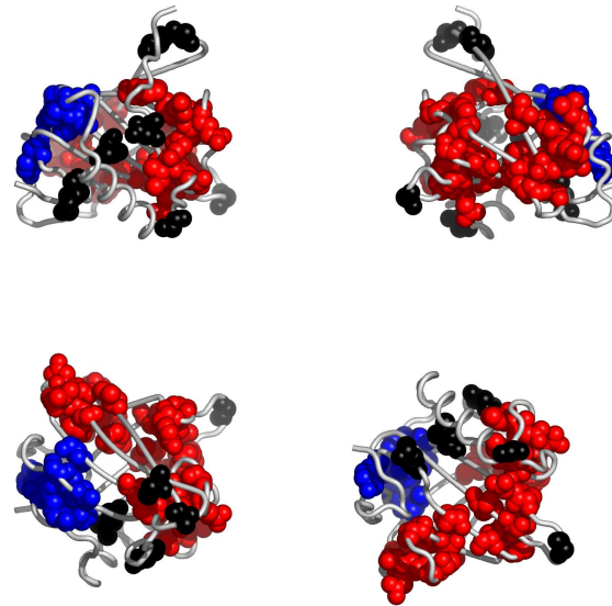
Fig. 3. Residues in li04A, colored according to the cluster they belong to: red, followed by blue and yellow are the largest clusters (see Appendix for the coloring scheme). Clockwise: front, back, top and bottom views. The corresponding Pymol script is attached.
