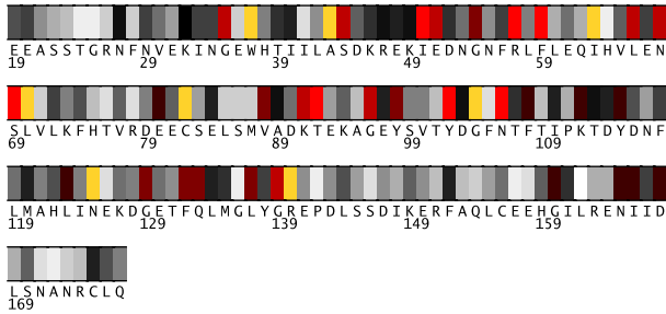
Fig. 1. Residues 19-177 in li04A colored by their relative importance. (See Appendix, Fig.5, for the coloring scheme.)
