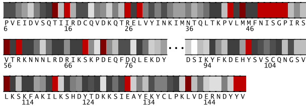
Fig. 1. Residues 6-150 in i13pA colored by their relative importance. (See Appendix, Fig.8, for the coloring scheme.)
