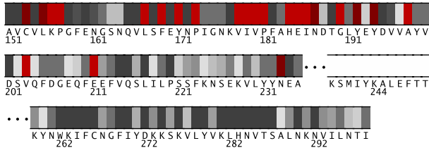
Fig. 2. Residues 151-298 in i13pA colored by their relative importance. (See Appendix, Fig.8, for the coloring scheme.)
