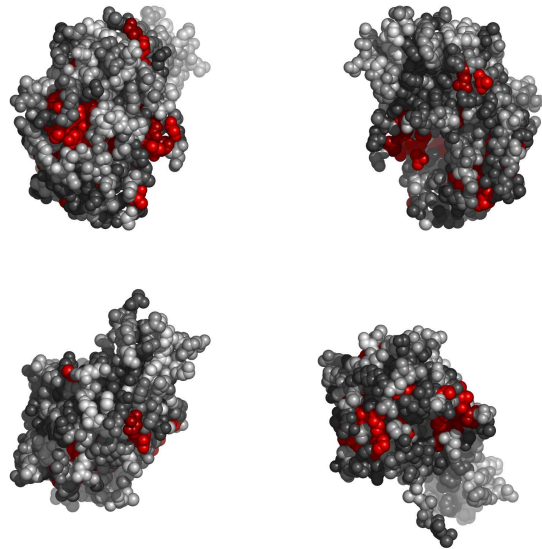
Fig. 3. Residues in i13pA, colored by their relative importance. Clockwise: front, back, top and bottom views.
