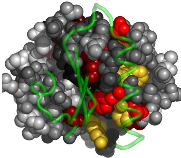
Fig. 5. Residues in lifqB, at the interface with lifqA, colored by their relative importance. lifqA is shown in backbone representation (See Appendix for the coloring scheme for the protein chain lifqB.)
