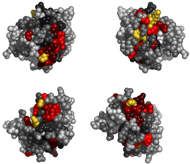
Fig. 2. Residues in lifqB, colored by their relative importance. Clockwise: front, back, top and bottom views.
