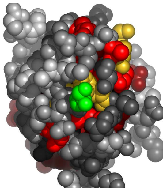
Fig. 4. Residues in 1lfqB, at the interface with glycerol, colored by their relative importance. The ligand (glycerol) is colored green. Atoms further than 30Å away from the geometric center of the ligand, as well as on the line of sight to the ligand were removed. (See Appendix for the coloring scheme for the protein chain 1lfqB.)
