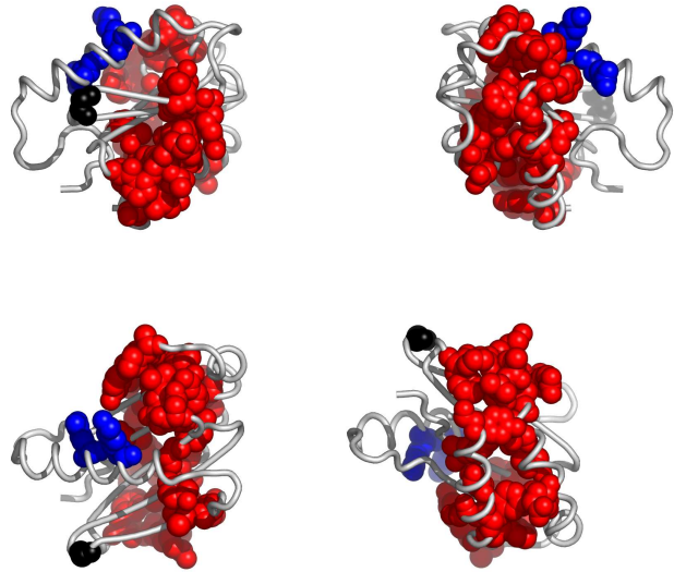
Fig. 3. Residues in lifqB, colored according to the cluster they belong to: red, followed by blue and yellow are the largest clusters (see Appendix for the coloring scheme). Clockwise: front, back, top and bottom views. The corresponding Pymol script is attached.
