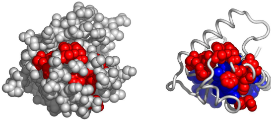
Fig. 5. Residues in lifqB, at the interface with lifqA, colored by their relative importance. lifqA is shown in backbone representation (See Appendix for the coloring scheme for the protein chain lifqB.)
