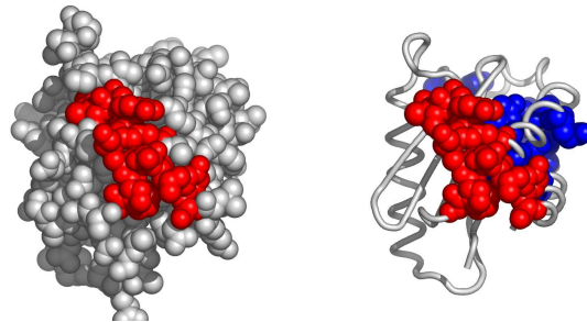
Fig. 7. Another possible active surface on the chain lifqB. The larger cluster it belongs to is shown in blue.
