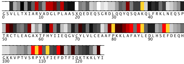
Fig. 1. Residues 0-127 in lifqB colored by their relative importance. (See Appendix, Fig.8, for the coloring scheme.)
