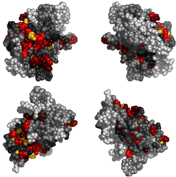
Fig. 3. Residues in lilgA, colored by their relative importance. Clockwise: front, back, top and bottom views.
