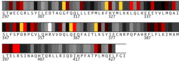
Fig. 2. Residues 297-431 in lilgA colored by their relative importance. (See Appendix, Fig.8, for the coloring scheme.)
