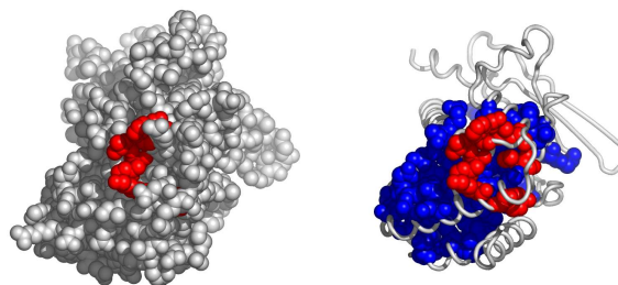
Fig. 7. Another possible active surface on the chain 1ilgA. The larger cluster it belongs to is shown in blue.
