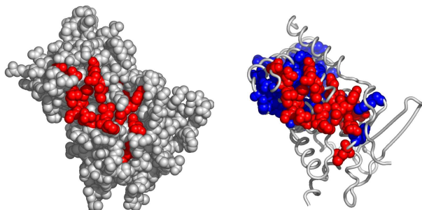
Fig. 5. A possible active surface on the chain 1ilgA. The larger cluster it belongs to is shown in blue.
