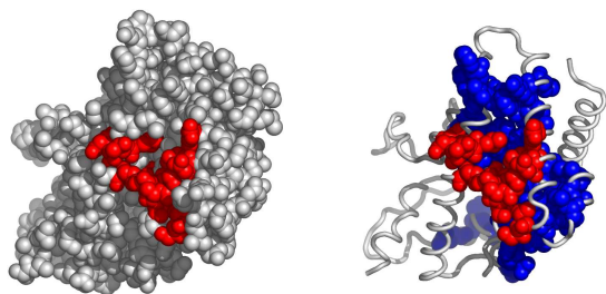
Fig. 6. Another possible active surface on the chain 1ilgA. The larger cluster it belongs to is shown in blue.
