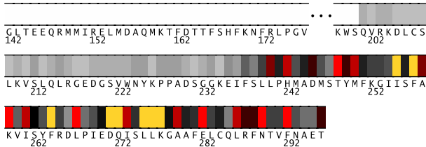
Fig. 1. Residues 142-296 in lilgA colored by their relative importance. (See Appendix, Fig.8, for the coloring scheme.)
