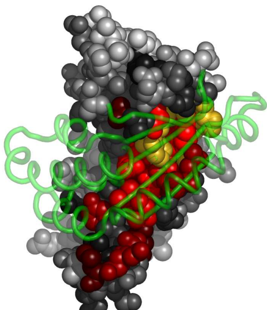
Fig. 4. Residues in 1j3mA, at the interface with 1j3mB, colored by their relative importance. 1j3mB is shown in backbone representation (See Appendix for the coloring scheme for the protein chain 1j3mA.)
