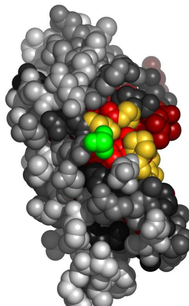
Fig. 5. Residues in 1j3mA, at the interface with sulfite ion, colored by their relative importance. The ligand (sulfite ion) is colored green. Atoms further than 30Å away from the geometric center of the ligand, as well as on the line of sight to the ligand were removed. (See Appendix for the coloring scheme for the protein chain 1j3mA.)
