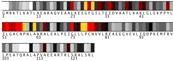
Fig. 1. Residues 3-129 in 1j3mA colored by their relative importance. (See Appendix, Fig.7, for the coloring scheme.)
