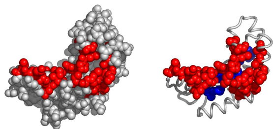
Fig. 6. A possible active surface on the chain 1j3mA. The larger cluster it belongs to is shown in blue.
