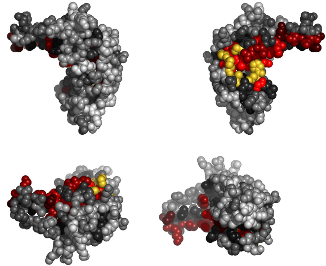
Fig. 1. Residues 3-129 in 1j3mA colored by their relative importance. (See Appendix, Fig.7, for the coloring scheme.)
