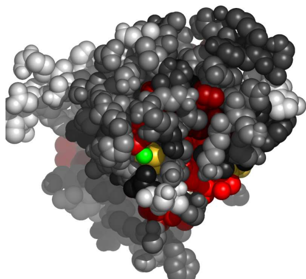
Fig. 5. Residues in 1j8fA, at the interface with zinc ion, colored by their relative importance. The ligand (zinc ion) is colored green. Atoms further than 30Å away from the geometric center of the ligand, as well as on the line of sight to the ligand were removed. (See Appendix for the coloring scheme for the protein chain 1j8fA.)
