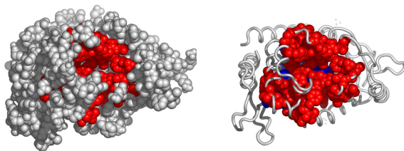
Fig. 6. A possible active surface on the chain 1j8fA. The larger cluster it belongs to is shown in blue.
