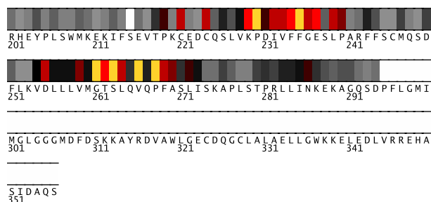
Fig. 2. Residues 201-356 in 1j8fA colored by their relative importance. (See Appendix, Fig.7, for the coloring scheme.)
