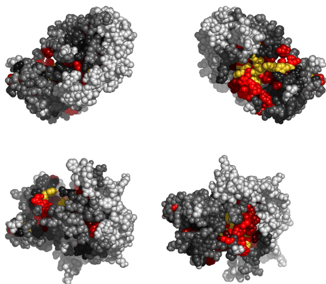
Fig. 3. Residues in 1j8fA, colored by their relative importance. Clockwise: front, back, top and bottom views.
