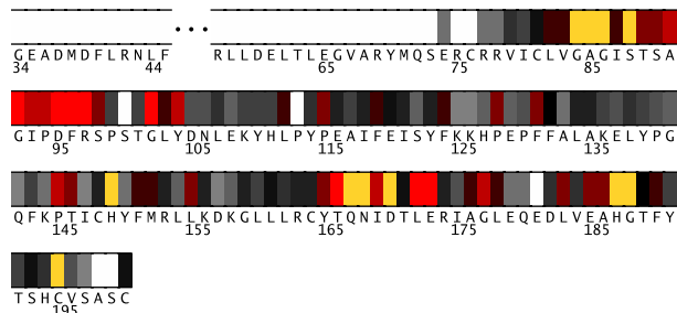
Fig. 1. Residues 34-200 in 1j8fA colored by their relative importance. (See Appendix, Fig.7, for the coloring scheme.)
