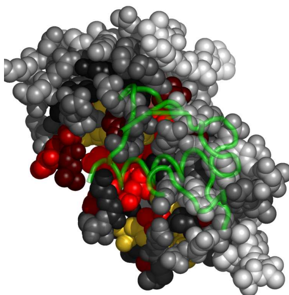
Fig. 4. Residues in 1jatA, at the interface with 1jatB, colored by their relative importance. 1jatB is shown in backbone representation (See Appendix for the coloring scheme for the protein chain 1jatA.)
