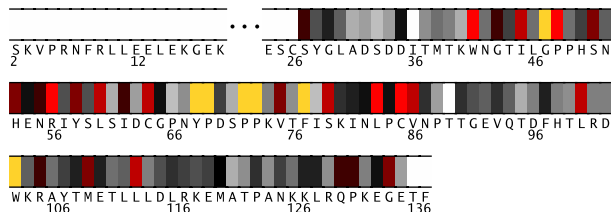
Fig. 6. Residues 2-137 in 1jatB colored by their relative importance. (See Appendix, Fig.11, for the coloring scheme.)
