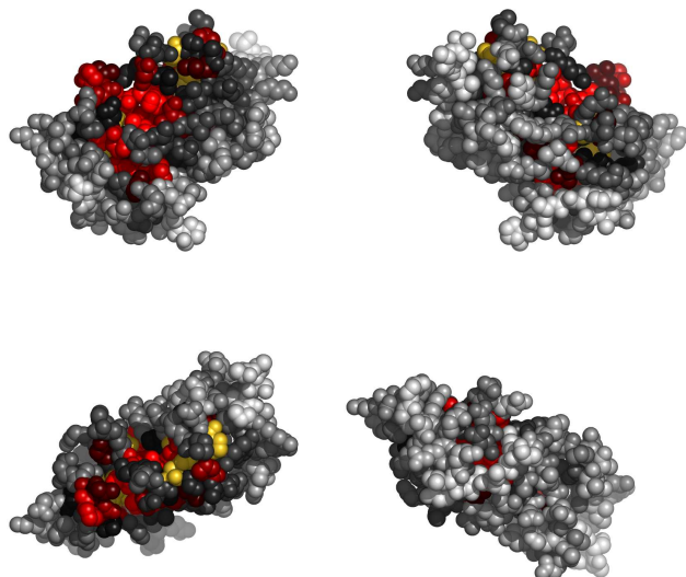
Fig. 1. Residues 1-152 in 1jatA colored by their relative importance. (See Appendix, Fig.11, for the coloring scheme.)
