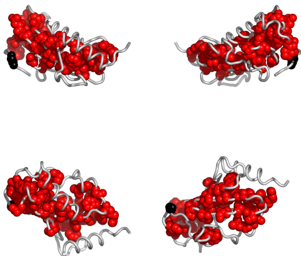
Fig. 8. Residues in 1jatB, colored according to the cluster they belong to: red, followed by blue and yellow are the largest clusters (see Appendix for the coloring scheme). Clockwise: front, back, top and bottom views. The corresponding Pymol script is attached.
