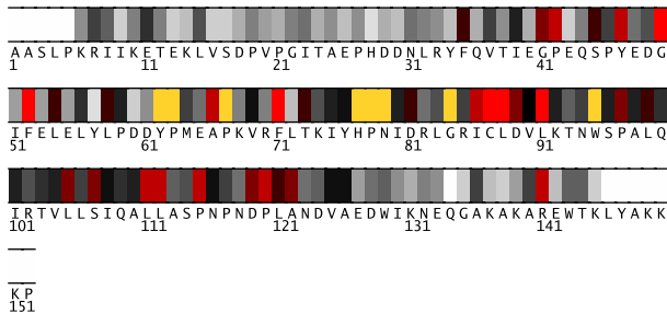
Fig. 1. Residues 1-152 in 1jatA colored by their relative importance. (See Appendix, Fig.11, for the coloring scheme.)
