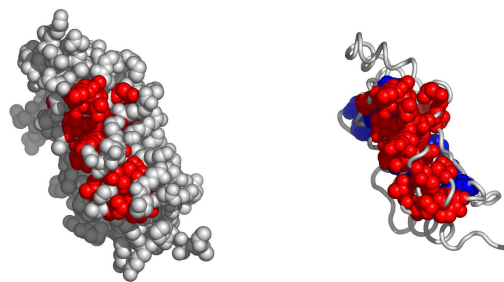
Fig. 5. A possible active surface on the chain 1jatA. The larger cluster it belongs to is shown in blue.
