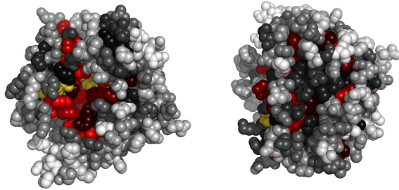
Fig. 3. Residues in 1jczA, colored by their relative importance. Clockwise: front, back, top and bottom views.
