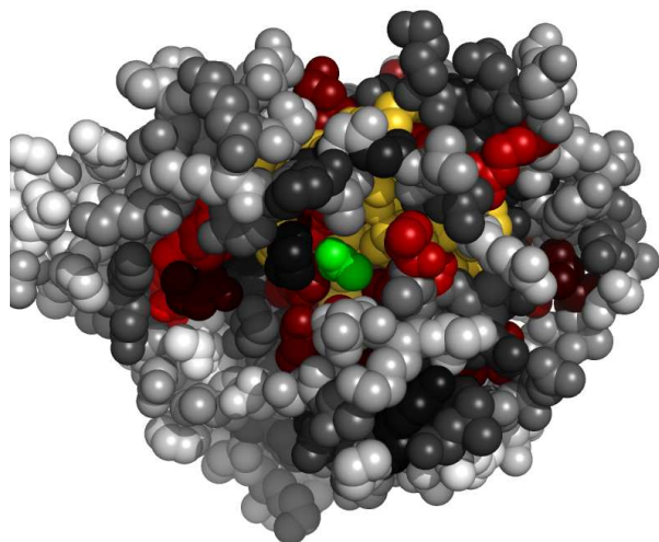
Fig. 7. Residues in 1jczA, at the interface with acetic acid, colored by their relative importance. The ligand (acetic acid) is colored green. Atoms further than 30\text{\AA} away from the geometric center of the ligand, as well as on the line of sight to the ligand were removed. (See Appendix for the coloring scheme for the protein chain 1jczA.)
