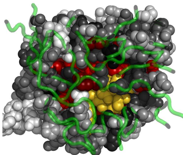
Fig. 6. Residues in 1jczA, at the interface with 1jczB, colored by their relative importance. 1jczB is shown in backbone representation (See Appendix for the coloring scheme for the protein chain 1jczA.)
