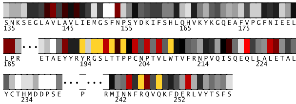
Fig. 2. Residues 135-261 in 1jczA colored by their relative importance. (See Appendix, Fig.8, for the coloring scheme.) Note that some residues in 1jczA carry insertion code.
