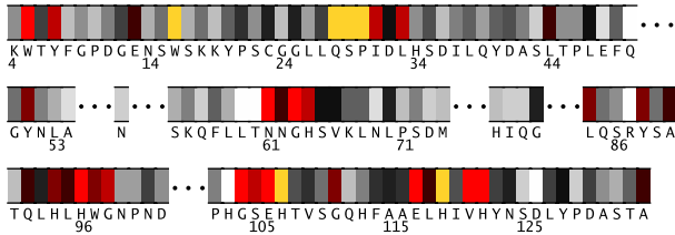
Fig. 1. Residues 4-134 in 1jczA colored by their relative importance. (See Appendix, Fig.8, for the coloring scheme.) Note that some residues in 1jczA carry insertion code.
