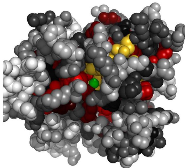
Fig. 5. Residues in 1jczA, at the interface with zinc ion, colored by their relative importance. The ligand (zinc ion) is colored green. Atoms further than 30Å away from the geometric center of the ligand, as well as on the line of sight to the ligand were removed. (See Appendix for the coloring scheme for the protein chain 1jczA.)
