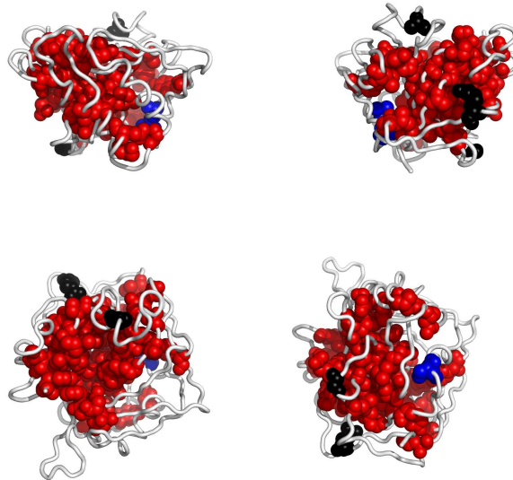
Fig. 4. Residues in 1jczA, colored according to the cluster they belong to: red, followed by blue and yellow are the largest clusters (see Appendix for the coloring scheme). Clockwise: front, back, top and bottom views. The corresponding Pymol script is attached.
