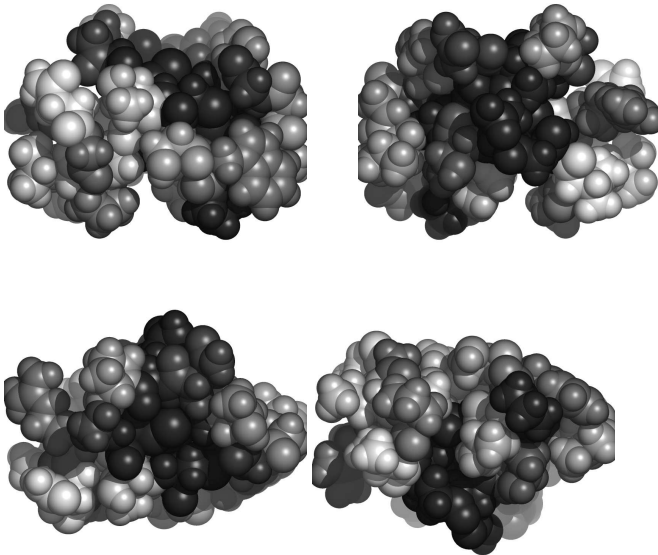
Fig. 2. Residues in 1jjzA, colored by their relative importance. Clockwise: front, back, top and bottom views.
