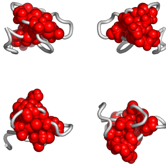
Fig. 3. Residues in 1jjzA, colored according to the cluster they belong to: red, followed by blue and yellow are the largest clusters (see Appendix for the coloring scheme). Clockwise: front, back, top and bottom views. The corresponding Pymol script is attached.
