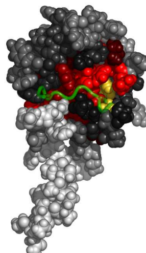
Fig. 4. Residues in 1ju5A, at the interface with 1ju5B, colored by their relative importance. 1ju5B is shown in backbone representation (See Appendix for the coloring scheme for the protein chain 1ju5A.)
