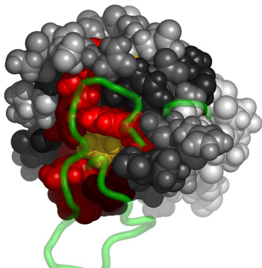
Fig. 10. Residues in 1ju5C, at the interface with 1ju5A, colored by their relative importance. 1ju5A is shown in backbone representation (See Appendix for the coloring scheme for the protein chain 1ju5C.)
