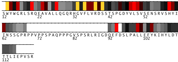
Fig. 1. Residues 12-120 in 1ju5A colored by their relative importance. (See Appendix, Fig.12, for the coloring scheme.)
