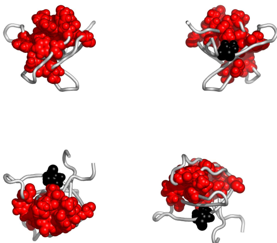
Fig. 9. Residues in 1ju5C, colored according to the cluster they belong to: red, followed by blue and yellow are the largest clusters (see Appendix for the coloring scheme). Clockwise: front, back, top and bottom views. The corresponding Pymol script is attached.
