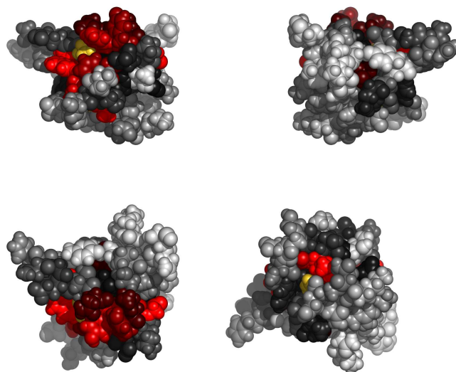
Fig. 8. Residues in 1ju5C, colored by their relative importance. Clockwise: front, back, top and bottom views.
