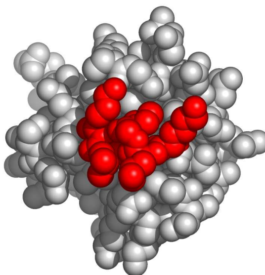
Fig. 5. Another possible active surface on the chain 1kw4A.
