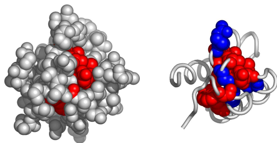
Fig. 4. A possible active surface on the chain 1kw4A. The larger cluster it belongs to is shown in blue.
