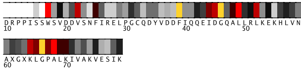
Fig. 1. Residues 10-79 in 1kw4A colored by their relative importance. (See Appendix, Fig.6, for the coloring scheme.)
