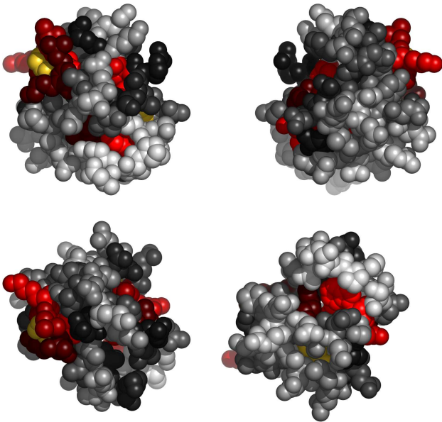
Fig. 2. Residues in 1kw4A, colored by their relative importance. Clockwise: front, back, top and bottom views.
