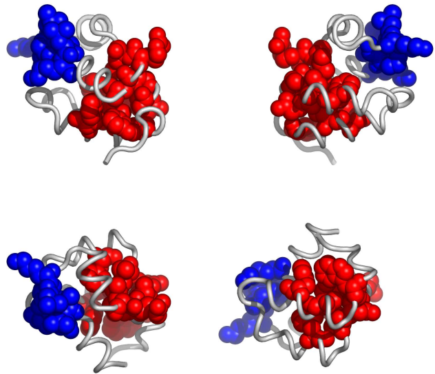
Fig. 1. Residues 10-79 in 1kw4A colored by their relative importance. (See Appendix, Fig.6, for the coloring scheme.)
