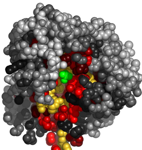
Fig. 5. Residues in 1lc5A, at the interface with phosphate ion, colored by their relative importance. The ligand (phosphate ion) is colored green. Atoms further than 30Å away from the geometric center of the ligand, as well as on the line of sight to the ligand were removed. (See Appendix for the coloring scheme for the protein chain 1lc5A.)
