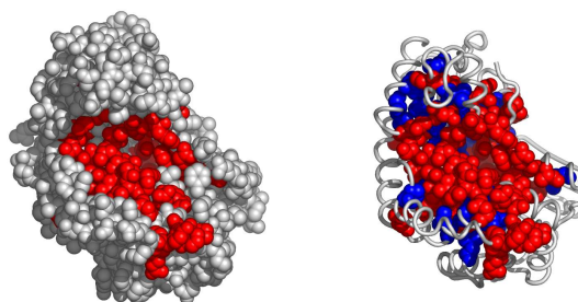
Fig. 7. Residues in 1lc5A, at the interface with 1lc5A1, colored by their relative importance. 1lc5A1 is shown in backbone representation (See Appendix for the coloring scheme for the protein chain 1lc5A.)
