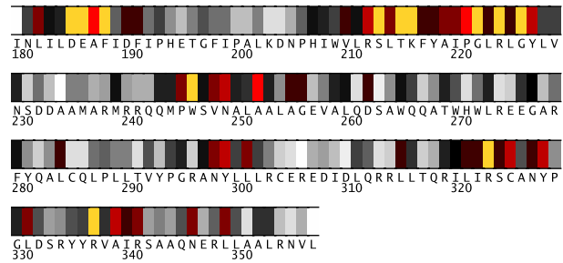
Fig. 2. Residues 180-357 in 1lc5A colored by their relative importance. (See Appendix, Fig.9, for the coloring scheme.)
