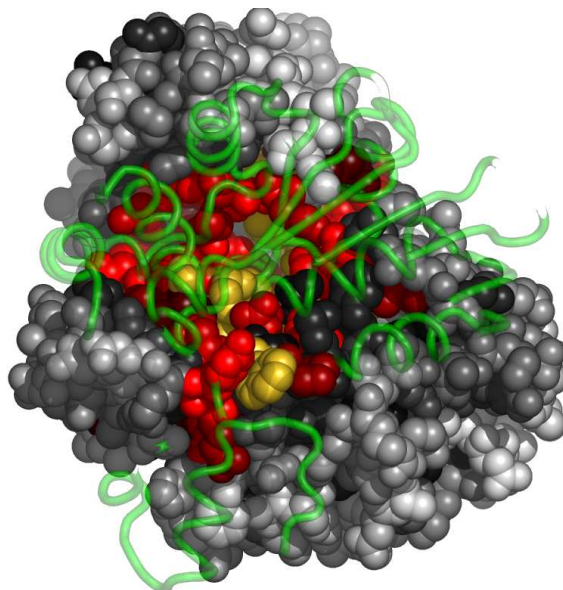
Fig. 7. Residues in 1lc5A, at the interface with 1lc5A1, colored by their relative importance. 1lc5A1 is shown in backbone representation (See Appendix for the coloring scheme for the protein chain 1lc5A.)
