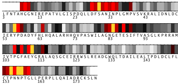
Fig. 1. Residues 3-179 in 1lc5A colored by their relative importance. (See Appendix, Fig.9, for the coloring scheme.)
