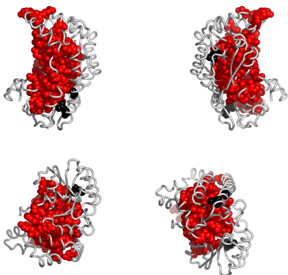
Fig. 4. Residues in 1lc5A, colored according to the cluster they belong to: red, followed by blue and yellow are the largest clusters (see Appendix for the coloring scheme). Clockwise: front, back, top and bottom views. The corresponding Pymol script is attached.
