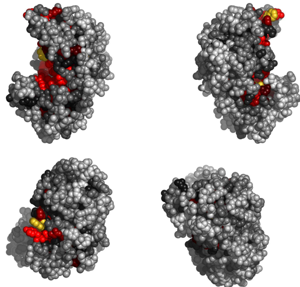
Fig. 3. Residues in 1lc5A, colored by their relative importance. Clockwise: front, back, top and bottom views.
