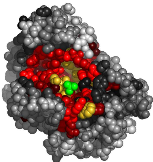
Fig. 6. Residues in 1lc5A, at the interface with phosphate ion, colored by their relative importance. The ligand (phosphate ion) is colored green. Atoms further than 30Å away from the geometric center of the ligand, as well as on the line of sight to the ligand were removed. (See Appendix for the coloring scheme for the protein chain 1lc5A.)
