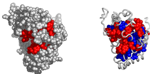
Fig. 7. A possible active surface on the chain 1110B. The larger cluster it belongs to is shown in blue.
