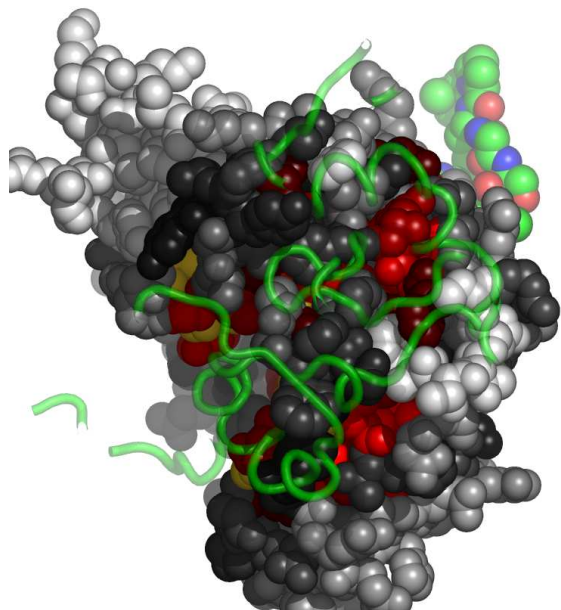
Fig. 6. Residues in 1110B, at the interface with 1110H, colored by their relative importance. 1110H is shown in backbone representation (See Appendix for the coloring scheme for the protein chain 1110B.)
