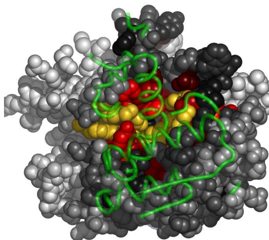
Fig. 4. Residues in 1110B, colored according to the cluster they belong to: red, followed by blue and yellow are the largest clusters (see Appendix for the coloring scheme). Clockwise: front, back, top and bottom views. The corresponding Pymol script is attached.
