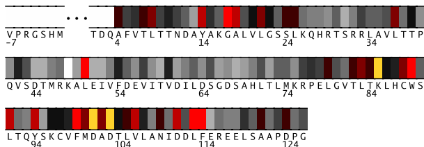
Fig. 1. Residues -7-126 in 1110B colored by their relative importance. (See Appendix, Fig.8, for the coloring scheme.)
