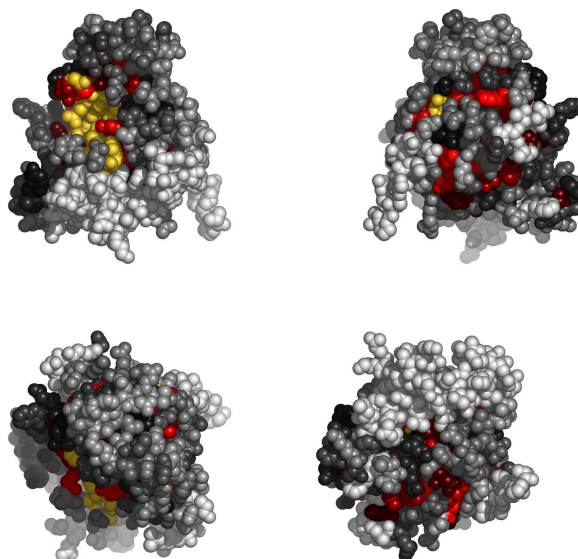
Fig. 3. Residues in 1110B, colored by their relative importance. Clockwise: front, back, top and bottom views.
