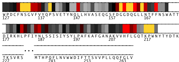
Fig. 2. Residues 127-266 in 1110B colored by their relative importance. (See Appendix, Fig.8, for the coloring scheme.)
