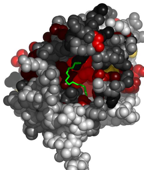
Fig. 5. Residues in 1lv2A, at the interface with palmitic acid, colored by their relative importance. The ligand (palmitic acid) is colored green. Atoms further than 30Å away from the geometric center of the ligand, as well as on the line of sight to the ligand were removed. (See Appendix for the coloring scheme for the protein chain 1lv2A.)
