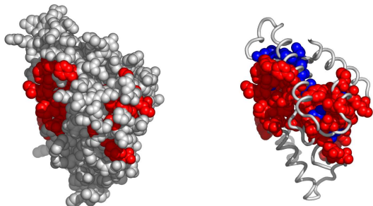
Fig. 6. A possible active surface on the chain 1lv2A. The larger cluster it belongs to is shown in blue.
