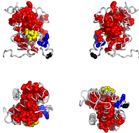
Fig. 3. Residues in 1lv2A, colored by their relative importance. Clockwise: front, back, top and bottom views.
