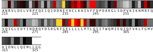
Fig. 2. Residues 215-327 in 1lv2A colored by their relative importance. (See Appendix, Fig.7, for the coloring scheme.)
