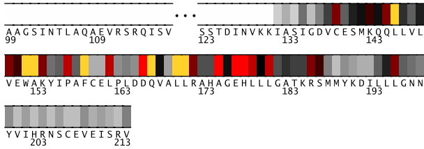
Fig. 1. Residues 99-214 in 1lv2A colored by their relative importance. (See Appendix, Fig.7, for the coloring scheme.)
