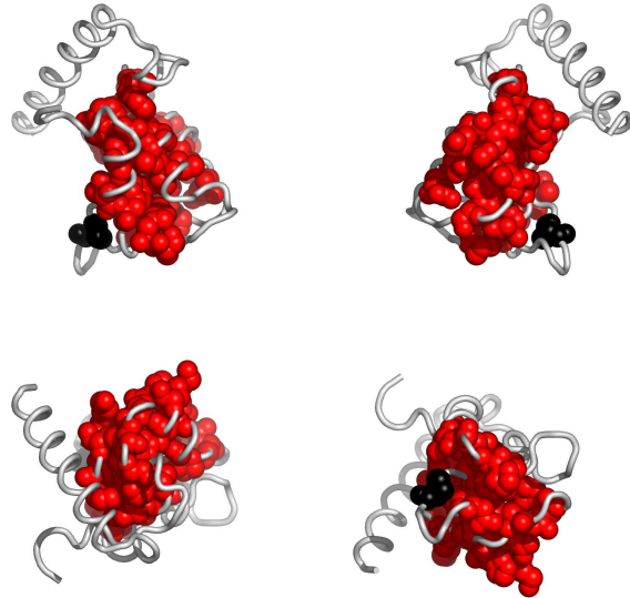
Fig. 3. Residues in 1m4mA, colored according to the cluster they belong to: red, followed by blue and yellow are the largest clusters (see Appendix for the coloring scheme). Clockwise: front, back, top and bottom views. The corresponding Pymol script is attached.
