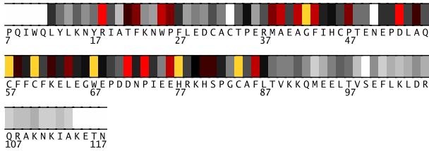
Fig. 1. Residues 7-118 in 1m4mA colored by their relative importance. (See Appendix, Fig.6, for the coloring scheme.)
