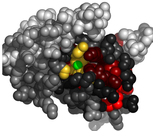
Fig. 5. Residues in 1m4mA, at the interface with zinc ion, colored by their relative importance. The ligand (zinc ion) is colored green. Atoms further than 30Å away from the geometric center of the ligand, as well as on the line of sight to the ligand were removed. (See Appendix for the coloring scheme for the protein chain 1m4mA.)
