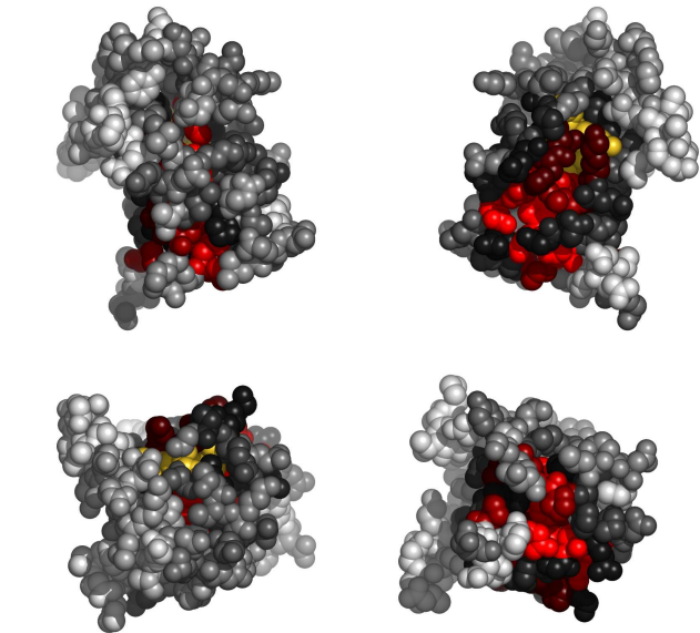
Fig. 1. Residues 7-118 in 1m4mA colored by their relative importance. (See Appendix, Fig.6, for the coloring scheme.)
