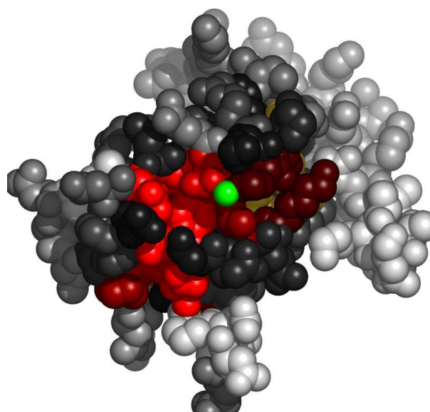
Fig. 4. Residues in 1m4mA, at the interface with zinc ion, colored by their relative importance. The ligand (zinc ion) is colored green. Atoms further than 30Å away from the geometric center of the ligand, as well as on the line of sight to the ligand were removed. (See Appendix for the coloring scheme for the protein chain 1m4mA.)
