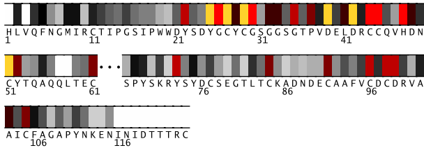
Fig. 1. Residues 1-124 in 1m8tF colored by their relative importance. (See Appendix, Fig.6, for the coloring scheme.)
