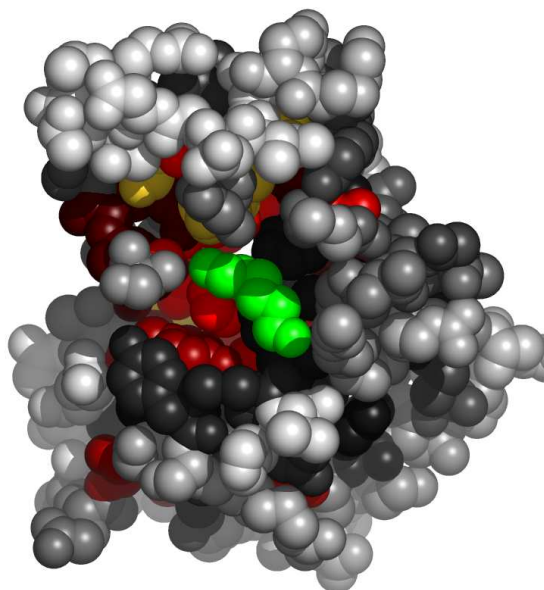
Fig. 4. Residues in 1m8tF, at the interface with hexane-1,6-diol, colored by their relative importance. The ligand (hexane-1,6-diol) is colored green. Atoms further than 30 Å away from the geometric center of the ligand, as well as on the line of sight to the ligand were removed. (See Appendix for the coloring scheme for the protein chain 1m8tF.)
