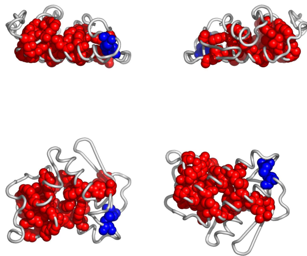
Fig. 3. Residues in 1m8tF, colored according to the cluster they belong to: red, followed by blue and yellow are the largest clusters (see Appendix for the coloring scheme). Clockwise: front, back, top and bottom views. The corresponding Pymol script is attached.
