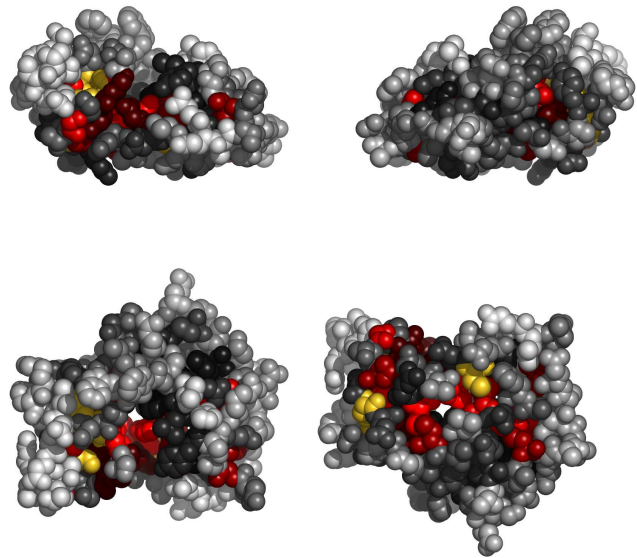
Fig. 2. Residues in 1m8tF, colored by their relative importance. Clockwise: front, back, top and bottom views.
