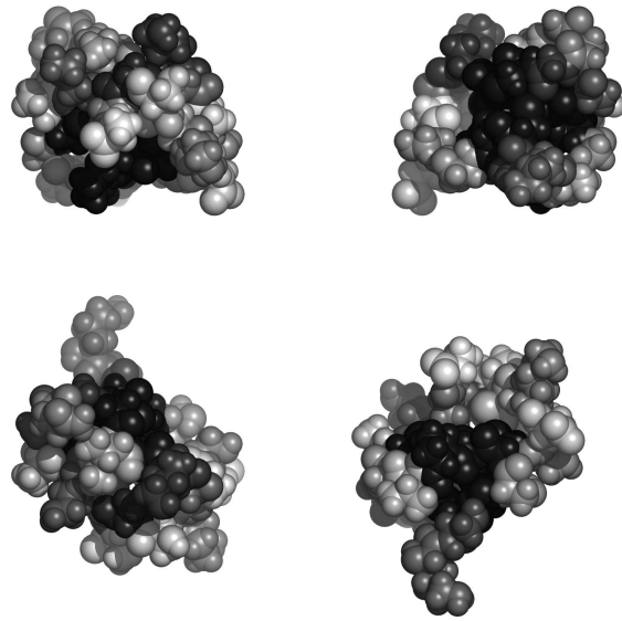
Fig. 2. Residues in 1mhuA, colored by their relative importance. Clockwise: front, back, top and bottom views.
