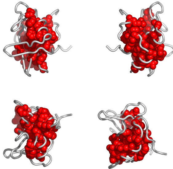
Fig. 3. Residues in 1milA, colored according to the cluster they belong to: red, followed by blue and yellow are the largest clusters (see Appendix for the coloring scheme). Clockwise: front, back, top and bottom views. The corresponding Pymol script is attached.
