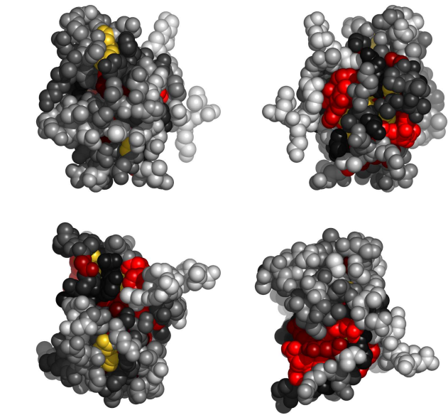
Fig. 2. Residues in 1milA, colored by their relative importance. Clockwise: front, back, top and bottom views.
