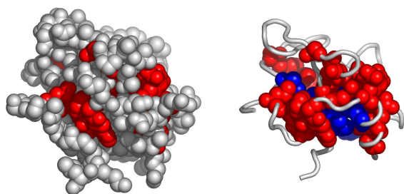
Fig. 4. A possible active surface on the chain 1milA. The larger cluster it belongs to is shown in blue.
