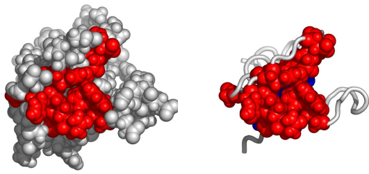
Fig. 4. A possible active surface on the chain 1muza. The larger cluster it belongs to is shown in blue.
