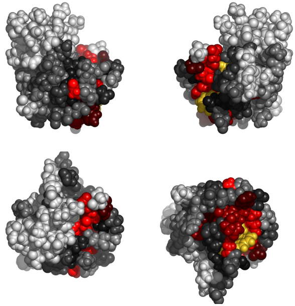
Fig. 2. Residues in 1muzA, colored by their relative importance. Clockwise: front, back, top and bottom views.
