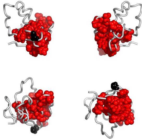
Fig. 3. Residues in 1muzA, colored according to the cluster they belong to: red, followed by blue and yellow are the largest clusters (see Appendix for the coloring scheme). Clockwise: front, back, top and bottom views. The corresponding Pymol script is attached.
