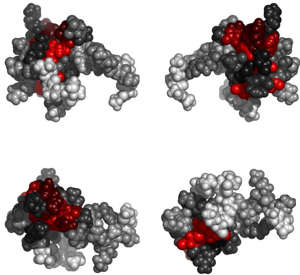
Fig. 2. Residues in 1n0zA, colored by their relative importance. Clockwise: front, back, top and bottom views.
