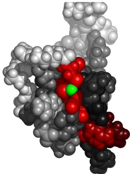
Fig. 4. Residues in 1n0zA, at the interface with zinc ion, colored by their relative importance. The ligand (zinc ion) is colored green. Atoms further than 30 Å away from the geometric center of the ligand, as well as on the line of sight to the ligand were removed. (See Appendix for the coloring scheme for the protein chain 1n0zA.)
