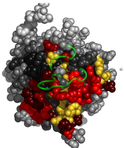
Fig. 7. Residues in 1o60A, at the interface with 1o60D, colored by their relative importance. 1o60D is shown in backbone representation (See Appendix for the coloring scheme for the protein chain 1o60A.)
