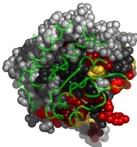
Fig. 6. Residues in 1o60A, at the interface with 1o60B, colored by their relative importance. 1o60B is shown in backbone representation (See Appendix for the coloring scheme for the protein chain 1o60A.)
