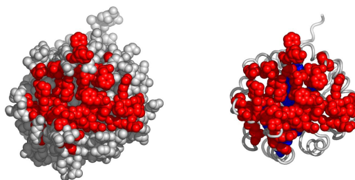
Fig. 8. A possible active surface on the chain 1o60A. The larger cluster it belongs to is shown in blue.
