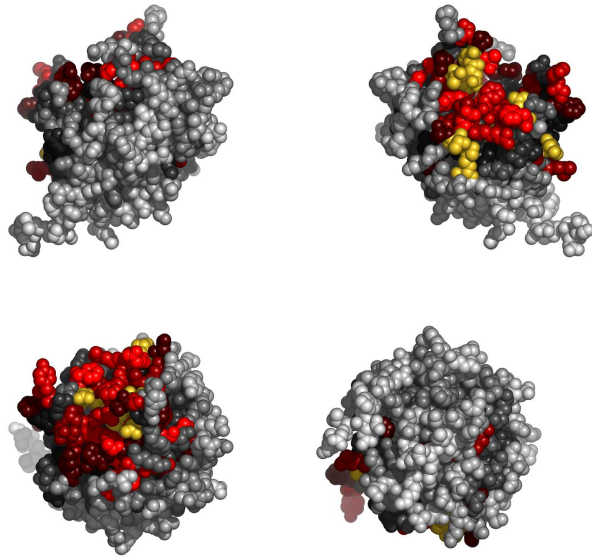
Fig. 3. Residues in 1o60A, colored by their relative importance. Clockwise: front, back, top and bottom views.
