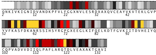
Fig. 1. Residues 2-135 in 1o60A colored by their relative importance. (See Appendix, Fig.9, for the coloring scheme.)
