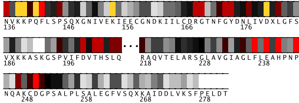
Fig. 2. Residues 136-282 in 1o60A colored by their relative importance. (See Appendix, Fig.9, for the coloring scheme.)
