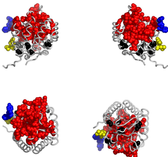
Fig. 4. Residues in 1o60A, colored according to the cluster they belong to: red, followed by blue and yellow are the largest clusters (see Appendix for the coloring scheme). Clockwise: front, back, top and bottom views. The corresponding Pymol script is attached.
