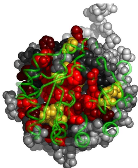
Fig. 5. Residues in 1o60A, at the interface with 1o60C, colored by their relative importance. 1o60C is shown in backbone representation (See Appendix for the coloring scheme for the protein chain 1o60A.)
