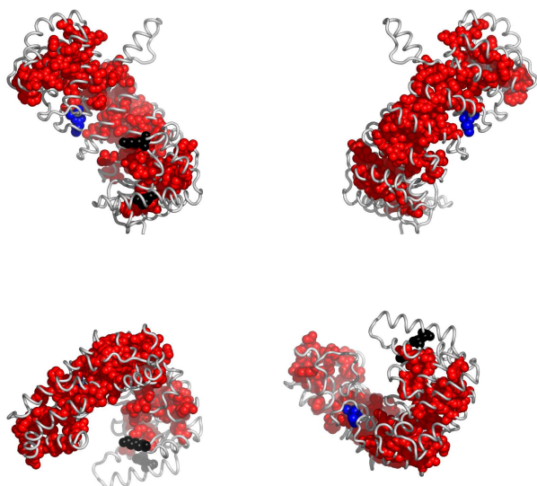
Fig. 4. Residues in 1o6oA, colored according to the cluster they belong to: red, followed by blue and yellow are the largest clusters (see Appendix for the coloring scheme). Clockwise: front, back, top and bottom views. The corresponding Pymol script is attached.
