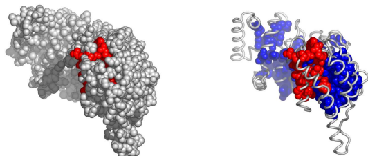
Fig. 9. Another possible active surface on the chain 1o6oA. The larger cluster it belongs to is shown in blue.
