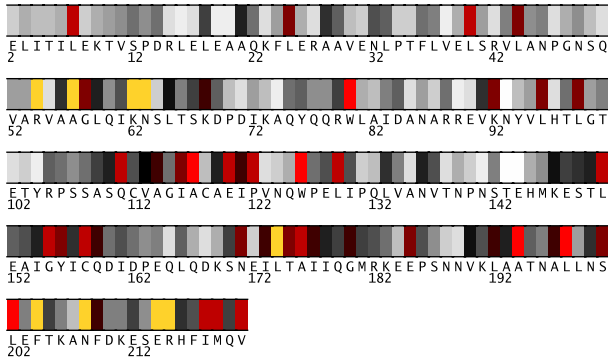
Fig. 1. Residues 2-221 in 1o6oA colored by their relative importance. (See Appendix, Fig.10, for the coloring scheme.)
