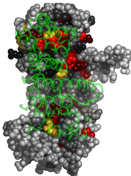
Fig. 6. Residues in 1o6oA, at the interface with 1o6oB, colored by their relative importance. 1o6oB is shown in backbone representation (See Appendix for the coloring scheme for the protein chain 1o6oA.)
