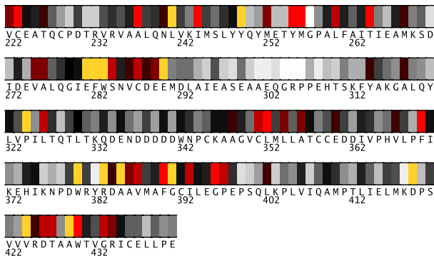
Fig. 2. Residues 222-441 in 1o6oA colored by their relative importance. (See Appendix, Fig.10, for the coloring scheme.)
