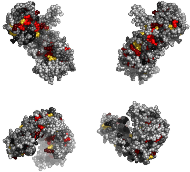
Fig. 3. Residues in 1o6oA, colored by their relative importance. Clockwise: front, back, top and bottom views.
