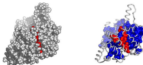
Fig. 6. Residues in 1o6oA, at the interface with 1o6oB, colored by their relative importance. 1o6oB is shown in backbone representation (See Appendix for the coloring scheme for the protein chain 1o6oA.)
