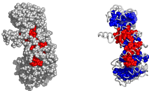
Fig. 8. Another possible active surface on the chain 1o6oA. The larger cluster it belongs to is shown in blue.
