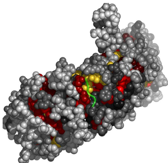
Fig. 5. Residues in 1o6oA, at the interface with 1o6oD, colored by their relative importance. 1o6oD is shown in backbone representation (See Appendix for the coloring scheme for the protein chain 1o6oA.)
