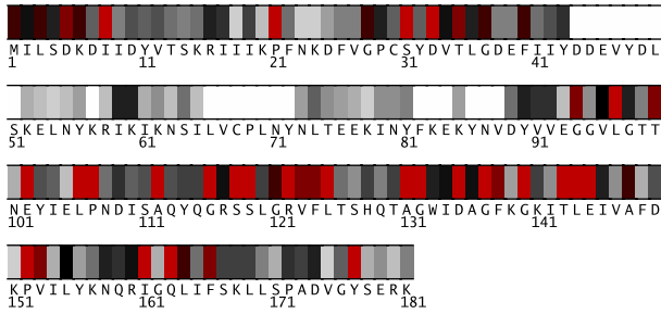
Fig. 1. Residues 1-181 in loghB colored by their relative importance. (See Appendix, Fig.7, for the coloring scheme.)
