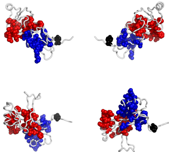
Fig. 3. Residues in loghB, colored according to the cluster they belong to: red, followed by blue and yellow are the largest clusters (see Appendix for the coloring scheme). Clockwise: front, back, top and bottom views. The corresponding Pymol script is attached.
