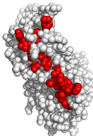
Fig. 6. Another possible active surface on the chain IoghB.
