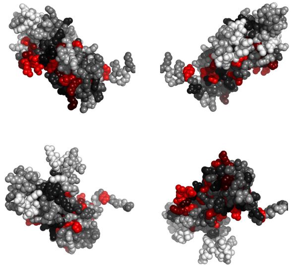
Fig. 2. Residues in loghB, colored by their relative importance. Clockwise: front, back, top and bottom views.
