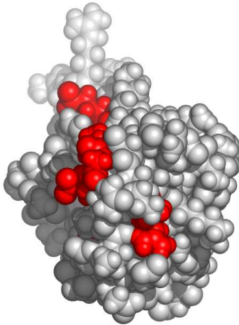
Fig. 4. Residues in loqpA, at the interface with loqpB, colored by their relative importance. loqpB is shown in backbone representation (See Appendix for the coloring scheme for the protein chain loqpA.)
