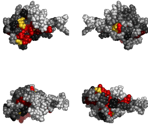
Fig. 1. Residues 93-169 in 1oqpA colored by their relative importance. (See Appendix, Fig.6, for the coloring scheme.)
