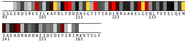
Fig. 1. Residues 93-169 in 1oqpA colored by their relative importance. (See Appendix, Fig.6, for the coloring scheme.)
