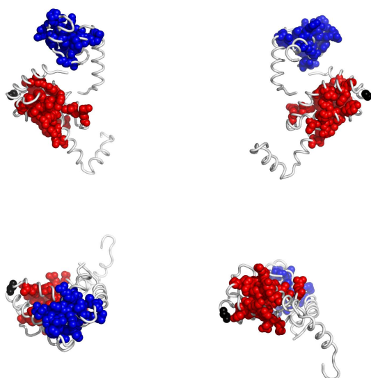
Fig. 6. Residues in 1or7A, colored according to the cluster they belong to: red, followed by blue and yellow are the largest clusters (see Appendix for the coloring scheme). Clockwise: front, back, top and bottom views. The corresponding Pymol script is attached.
