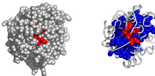
Fig. 6. A possible active surface on the chain 1p5jA. The larger cluster it belongs to is shown in blue.
