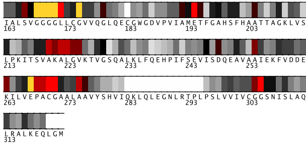
Fig. 2. Residues 163-322 in 1p5jA colored by their relative importance. (See Appendix, Fig.8, for the coloring scheme.)
