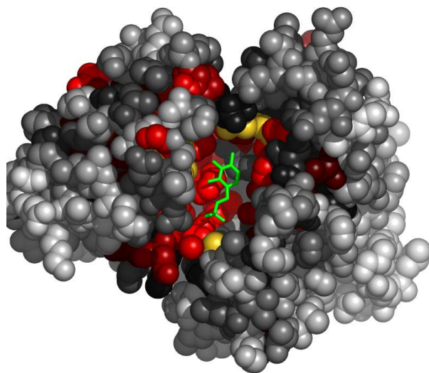
Fig. 5. Residues in 1p5jA, at the interface with PLP, colored by their relative importance. The ligand (PLP) is colored green. Atoms further than 30Å away from the geometric center of the ligand, as well as on the line of sight to the ligand were removed. (See Appendix for the coloring scheme for the protein chain 1p5jA.)
