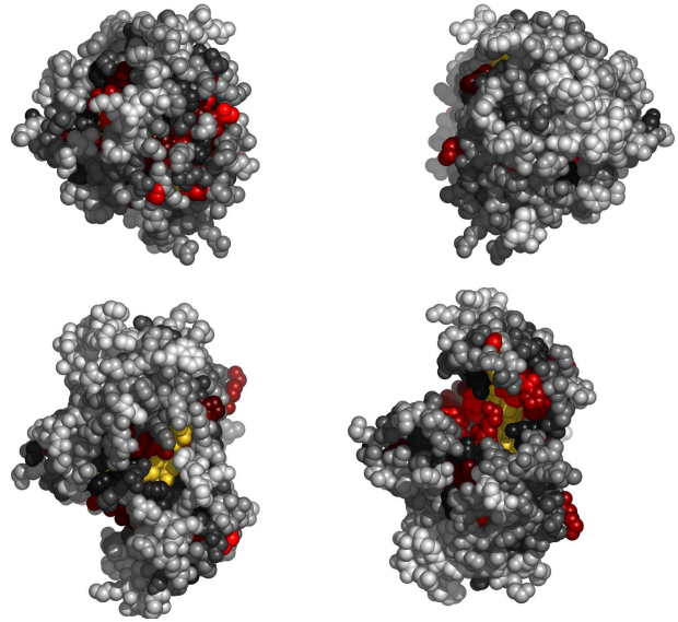
Fig. 3. Residues in 1p5jA, colored by their relative importance. Clockwise: front, back, top and bottom views.
