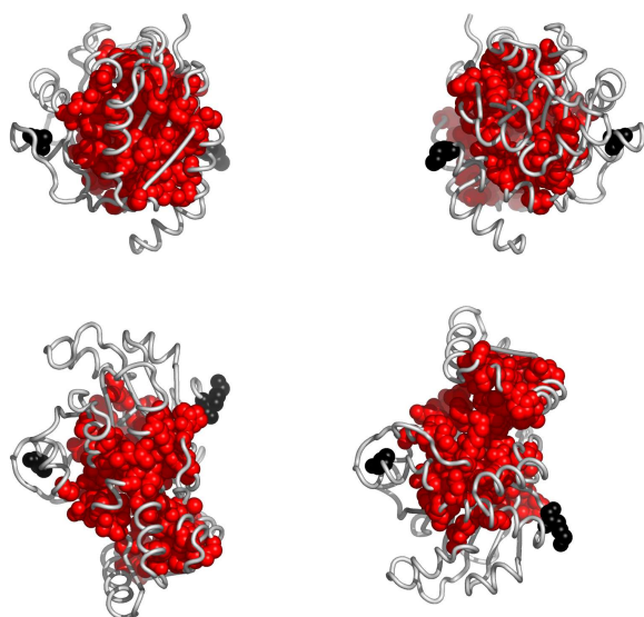
Fig. 4. Residues in 1p5jA, colored according to the cluster they belong to: red, followed by blue and yellow are the largest clusters (see Appendix for the coloring scheme). Clockwise: front, back, top and bottom views. The corresponding Pymol script is attached.
