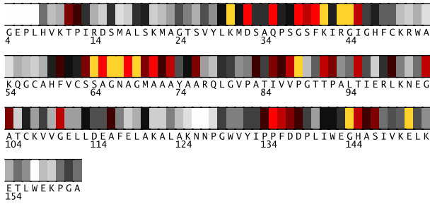
Fig. 1. Residues 4-162 in 1p5jA colored by their relative importance. (See Appendix, Fig.8, for the coloring scheme.)
