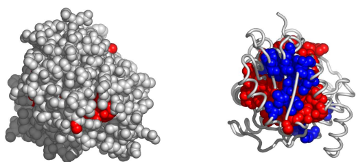
Fig. 7. Another possible active surface on the chain 1p5jA. The larger cluster it belongs to is shown in blue.
