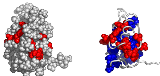
Fig. 5. Another possible active surface on the chain 1p97A. The larger cluster it belongs to is shown in blue.
