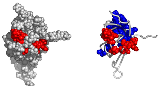
Fig. 4. A possible active surface on the chain 1p97A. The larger cluster it belongs to is shown in blue.
