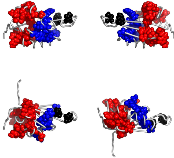
Fig. 3. Residues in 1p97A, colored according to the cluster they belong to: red, followed by blue and yellow are the largest clusters (see Appendix for the coloring scheme). Clockwise: front, back, top and bottom views. The corresponding Pymol script is attached.
