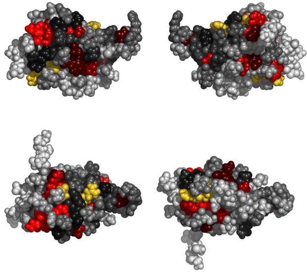
Fig. 2. Residues in 1p97A, colored by their relative importance. Clockwise: front, back, top and bottom views.
