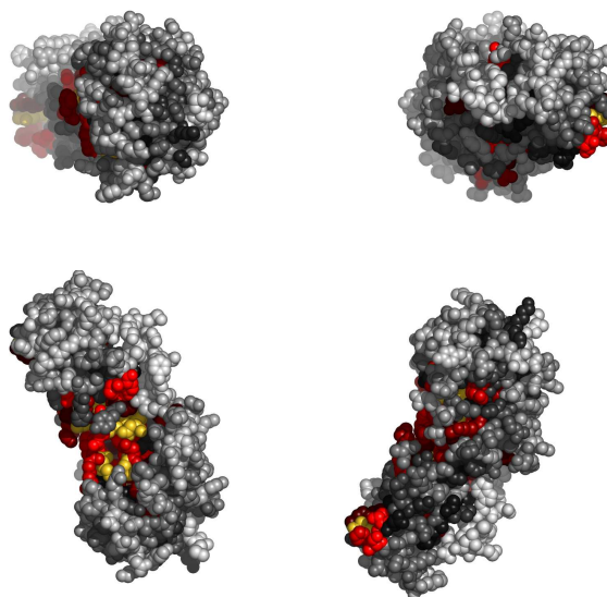
Fig. 3. Residues in 1pfkA, colored by their relative importance. Clockwise: front, back, top and bottom views.
