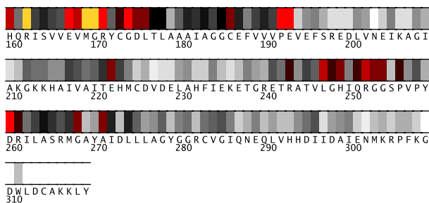
Fig. 2. Residues 160-319 in 1pfkA colored by their relative importance. (See Appendix, Fig.14, for the coloring scheme.)
