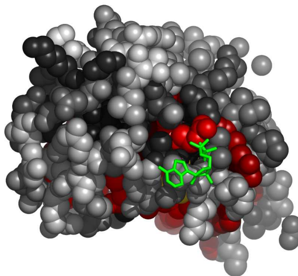
Fig. 6. Residues in 1pfkA, at the interface with ADP, colored by their relative importance. The ligand (ADP) is colored green. Atoms further than 30Å away from the geometric center of the ligand, as well as on the line of sight to the ligand were removed. (See Appendix for the coloring scheme for the protein chain 1pfkA.)
