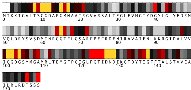
Fig. 1. Residues 0-159 in 1pfkA colored by their relative importance. (See Appendix, Fig.14, for the coloring scheme.)
