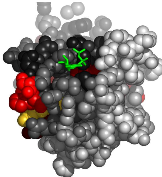
Fig. 7. Residues in 1pfkA, at the interface with ADP, colored by their relative importance. The ligand (ADP) is colored green. Atoms further than 30Å away from the geometric center of the ligand, as well as on the line of sight to the ligand were removed. (See Appendix for the coloring scheme for the protein chain 1pfkA.)
