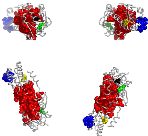
Fig. 4. Residues in 1pfaA, colored according to the cluster they belong to: red, followed by blue and yellow are the largest clusters (see Appendix for the coloring scheme). Clockwise: front, back, top and bottom views. The corresponding Pymol script is attached.
