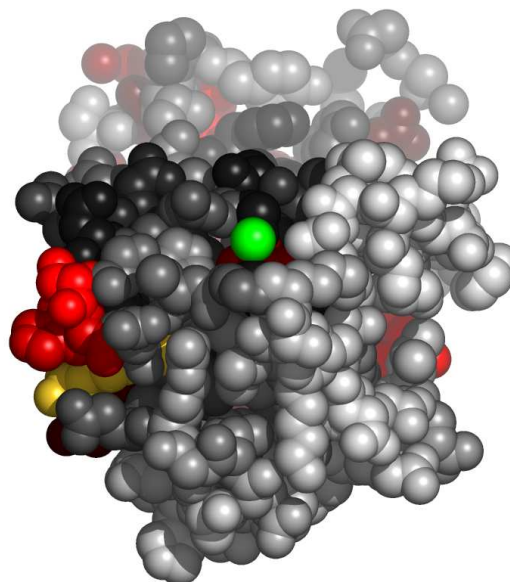
Fig. 9. Residues in 1pfa, at the interface with magnesium ion, colored by their relative importance. The ligand (magnesium ion) is colored green. Atoms further than 30Å away from the geometric center of the ligand, as well as on the line of sight to the ligand were removed. (See Appendix for the coloring scheme for the protein chain 1pfa.)
