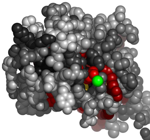
Fig. 11. Residues in 1pfkA, at the interface with magnesium ion, colored by their relative importance. The ligand (magnesium ion) is colored green. Atoms further than 30 Å away from the geometric center of the ligand, as well as on the line of sight to the ligand were removed. (See Appendix for the coloring scheme for the protein chain 1pfkA.)
