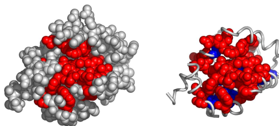
Fig. 5. A possible active surface on the chain 1pq1A. The larger cluster it belongs to is shown in blue.
