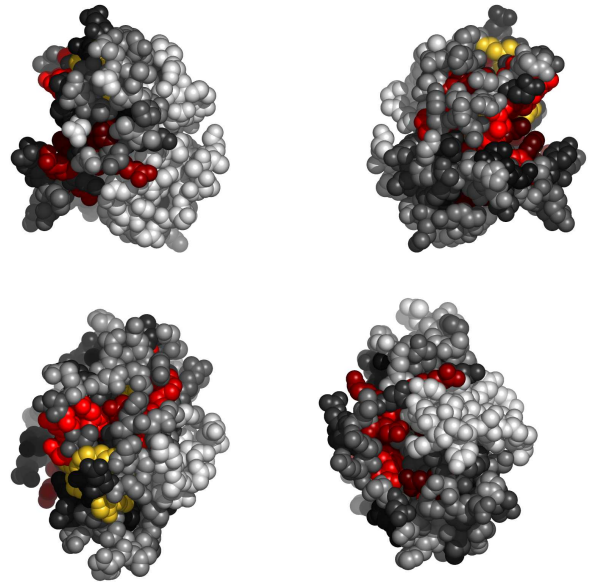
Fig. 2. Residues in 1pq1A, colored by their relative importance. Clockwise: front, back, top and bottom views.
