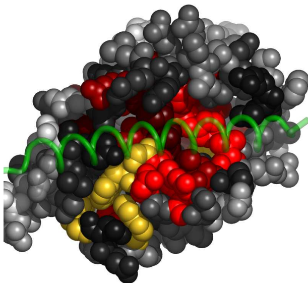
Fig. 4. Residues in 1pq1A, at the interface with 1pq1B, colored by their relative importance. 1pq1B is shown in backbone representation (See Appendix for the coloring scheme for the protein chain 1pq1A.)
