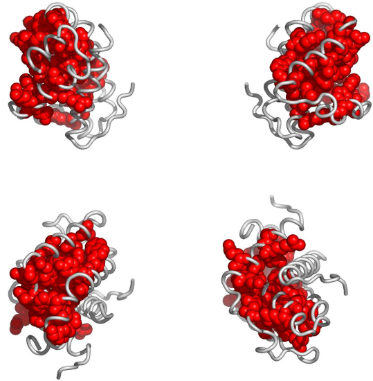
Fig. 3. Residues in 1pq1A, colored according to the cluster they belong to: red, followed by blue and yellow are the largest clusters (see Appendix for the coloring scheme). Clockwise: front, back, top and bottom views. The corresponding Pymol script is attached.
