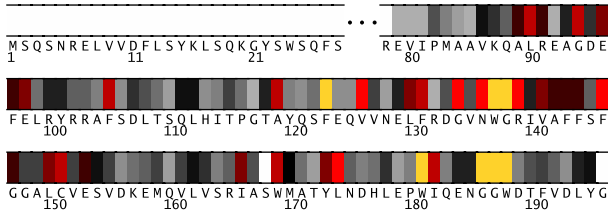
Fig. 1. Residues 1-196 in 1pq1A colored by their relative importance. (See Appendix, Fig.6, for the coloring scheme.)
