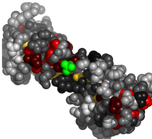
Fig. 4. Residues in 1qg3A, at the interface with sulfate ion, colored by their relative importance. The ligand (sulfate ion) is colored green. Atoms further than 30Å away from the geometric center of the ligand, as well as on the line of sight to the ligand were removed. (See Appendix for the coloring scheme for the protein chain 1qg3A.)
