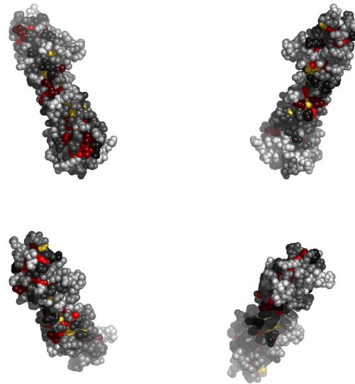
Fig. 2. Residues in 1qg3A, colored by their relative importance. Clockwise: front, back, top and bottom views.
