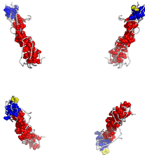
Fig. 2. Residues in 1qg3A, colored by their relative importance. Clockwise: front, back, top and bottom views.
