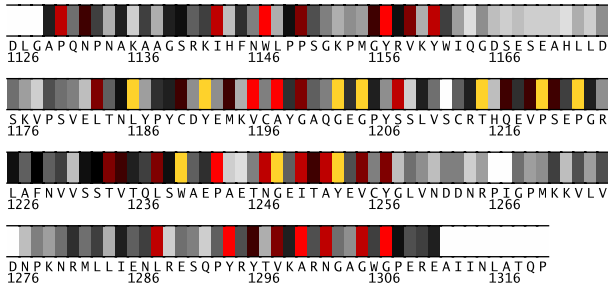
Fig. 1. Residues 1126-1320 in 1qg3A colored by their relative importance. (See Appendix, Fig.9, for the coloring scheme.)
