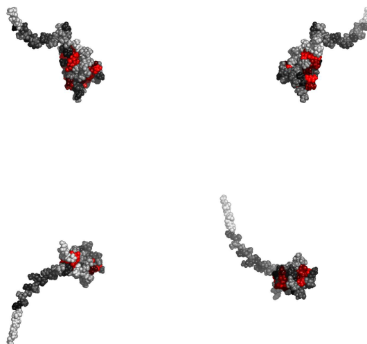
Fig. 2. Residues in 1r79A, colored by their relative importance. Clockwise: front, back, top and bottom views.
