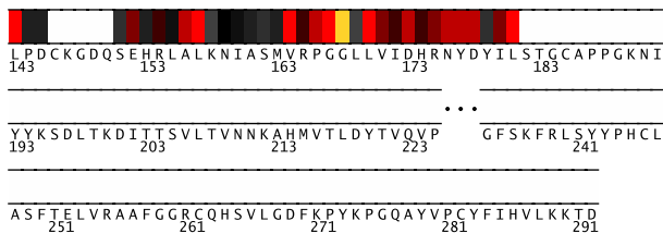
Fig. 2. Residues 143-292 in 1r8xB colored by their relative importance. (See Appendix, Fig.10, for the coloring scheme.)
