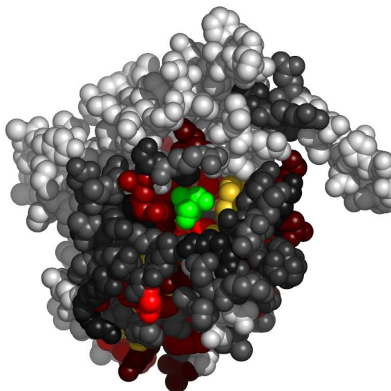
Fig. 7. Residues in 1r8xB, at the interface with TRS, colored by their relative importance. The ligand (TRS) is colored green. Atoms further than 30Å away from the geometric center of the ligand, as well as on the line of sight to the ligand were removed. (See Appendix for the coloring scheme for the protein chain 1r8xB.)
