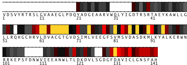
Fig. 1. Residues 1-142 in 1r8xB colored by their relative importance. (See Appendix, Fig.10, for the coloring scheme.)
