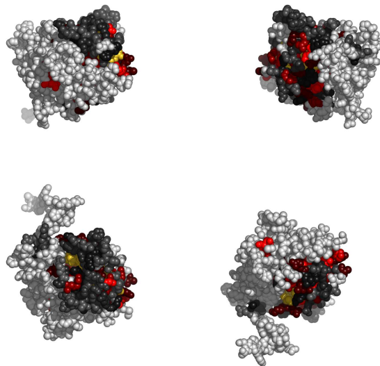
Fig. 3. Residues in 1r8xB, colored by their relative importance. Clockwise: front, back, top and bottom views.
