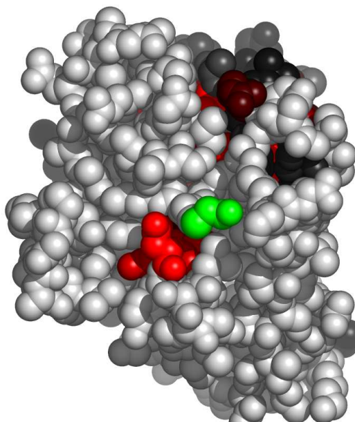
Fig. 5. Residues in 1r8xB, at the interface with beta-mercaptoethanol, colored by their relative importance. The ligand (beta-mercaptoethanol) is colored green. Atoms further than 30 Å away from the geometric center of the ligand, as well as on the line of sight to the ligand were removed. (See Appendix for the coloring scheme for the protein chain 1r8xB.)
