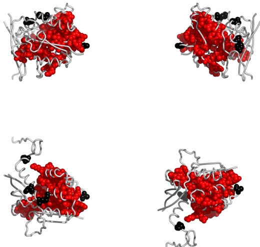
Fig. 4. Residues in 1r8xB, colored according to the cluster they belong to: red, followed by blue and yellow are the largest clusters (see Appendix for the coloring scheme). Clockwise: front, back, top and bottom views. The corresponding Pymol script is attached.
