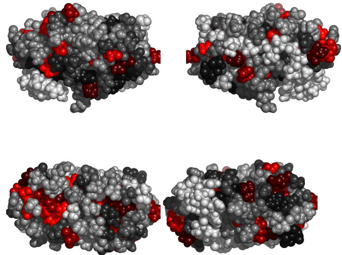
Fig. 1. Residues 1-143 in 1rx1A colored by their relative importance. (See Appendix, Fig.5, for the coloring scheme.)
