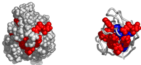
Fig. 4. A possible active surface on the chain 1rx1A. The larger cluster it belongs to is shown in blue.
