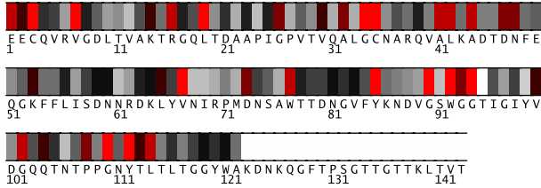
Fig. 1. Residues 1-143 in 1rx1A colored by their relative importance. (See Appendix, Fig.5, for the coloring scheme.)
