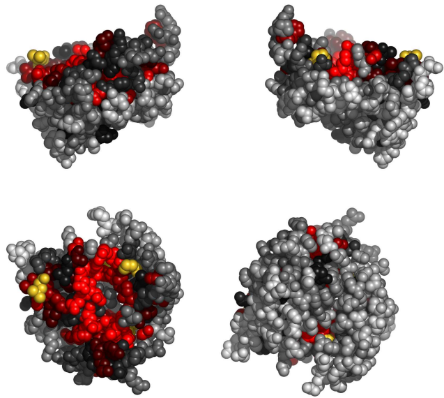
Fig. 2. Residues in 1s14B, colored by their relative importance. Clockwise: front, back, top and bottom views.
