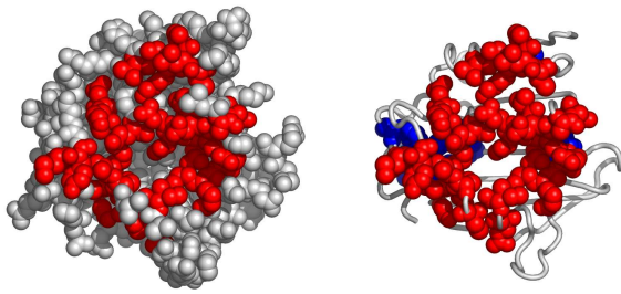
Fig. 5. A possible active surface on the chain 1s14B. The larger cluster it belongs to is shown in blue.
