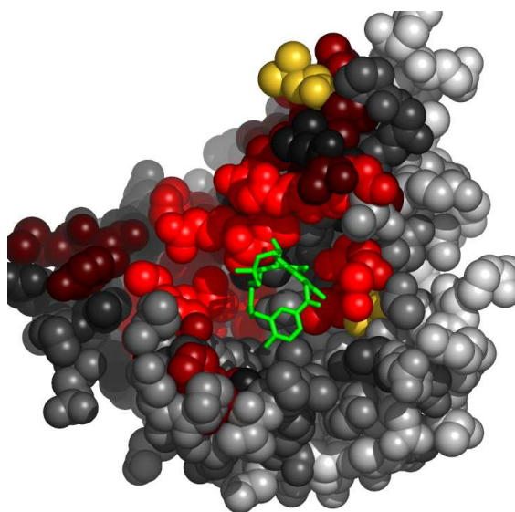
Fig. 4. Residues in 1s14B, at the interface with novobiocin, colored by their relative importance. The ligand (novobiocin) is colored green. Atoms further than 30 Å away from the geometric center of the ligand, as well as on the line of sight to the ligand were removed. (See Appendix for the coloring scheme for the protein chain 1s14B.)
