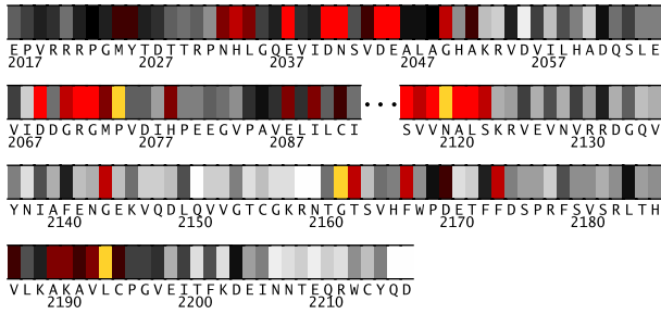
Fig. 1. Residues 2017-2217 in 1s14B colored by their relative importance. (See Appendix, Fig.6, for the coloring scheme.)
