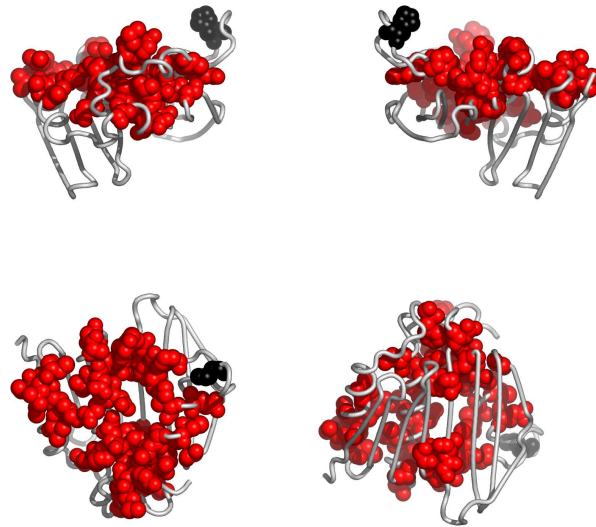
Fig. 3. Residues in 1s14B, colored according to the cluster they belong to: red, followed by blue and yellow are the largest clusters (see Appendix for the coloring scheme). Clockwise: front, back, top and bottom views. The corresponding Pymol script is attached.
