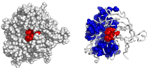
Fig. 5. A possible active surface on the chain 1s4uX. The larger cluster it belongs to is shown in blue.
