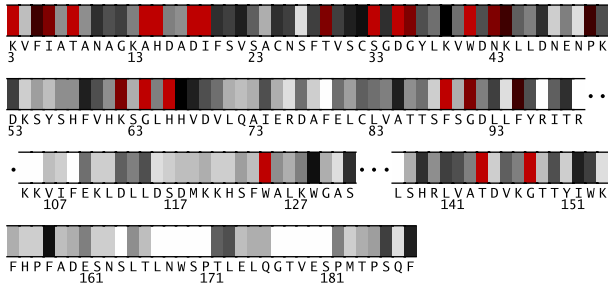
Fig. 1. Residues 3-188 in 1s4uX colored by their relative importance. (See Appendix, Fig.8, for the coloring scheme.)
