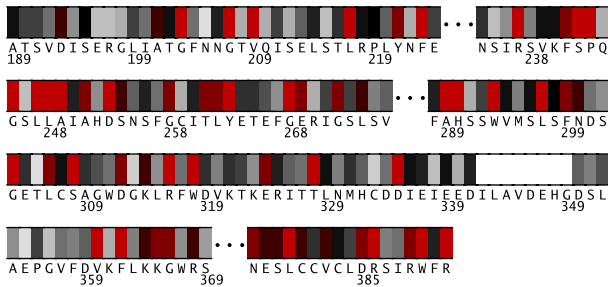
Fig. 2. Residues 189-392 in 1s4uX colored by their relative importance. (See Appendix, Fig.8, for the coloring scheme.)
