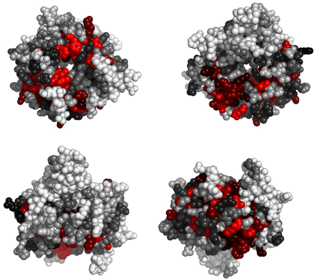
Fig. 3. Residues in 1s4uX, colored by their relative importance. Clockwise: front, back, top and bottom views.
