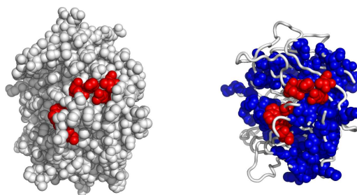
Fig. 7. Another possible active surface on the chain 1s4uX. The larger cluster it belongs to is shown in blue.
