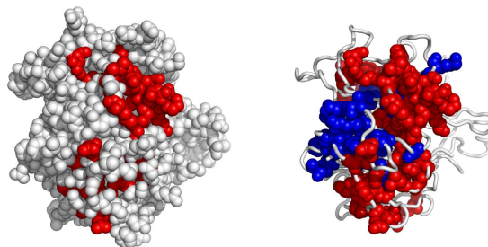
Fig. 6. Another possible active surface on the chain 1s4uX. The larger cluster it belongs to is shown in blue.
