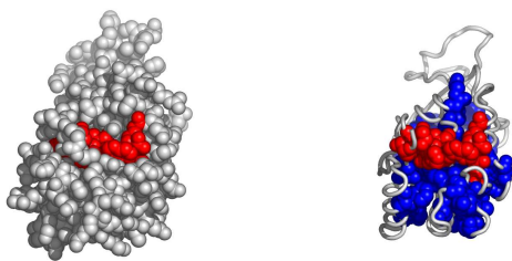
Fig. 6. A possible active surface on the chain 1t29A. The larger cluster it belongs to is shown in blue.
