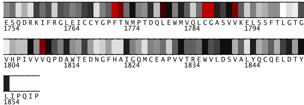
Fig. 2. Residues 1754-1859 in 1t29A colored by their relative importance. (See Appendix, Fig.8, for the coloring scheme.)
