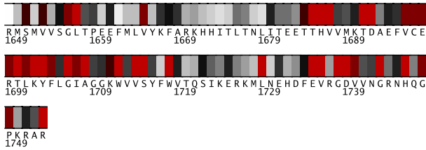
Fig. 1. Residues 1649-1753 in 1t29A colored by their relative importance. (See Appendix, Fig.8, for the coloring scheme.)
