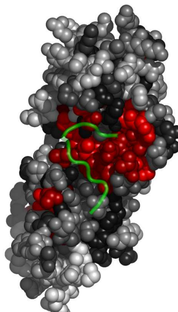
Fig. 5. Residues in 1t29A, at the interface with 1t29B, colored by their relative importance. 1t29B is shown in backbone representation (See Appendix for the coloring scheme for the protein chain 1t29A.)
