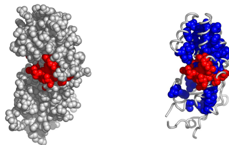
Fig. 7. Another possible active surface on the chain 1t29A. The larger cluster it belongs to is shown in blue.
