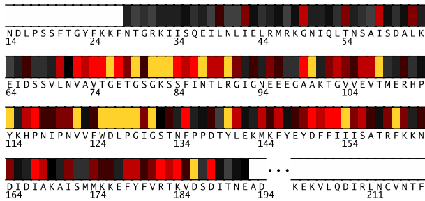
Fig. 1. Residues 14-217 in ItpzA colored by their relative importance. (See Appendix, Fig.10, for the coloring scheme.)
