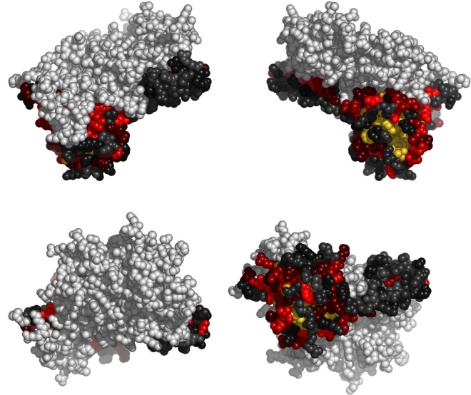
Fig. 1. Residues 14-217 in ItpzA colored by their relative importance. (See Appendix, Fig.10, for the coloring scheme.)
