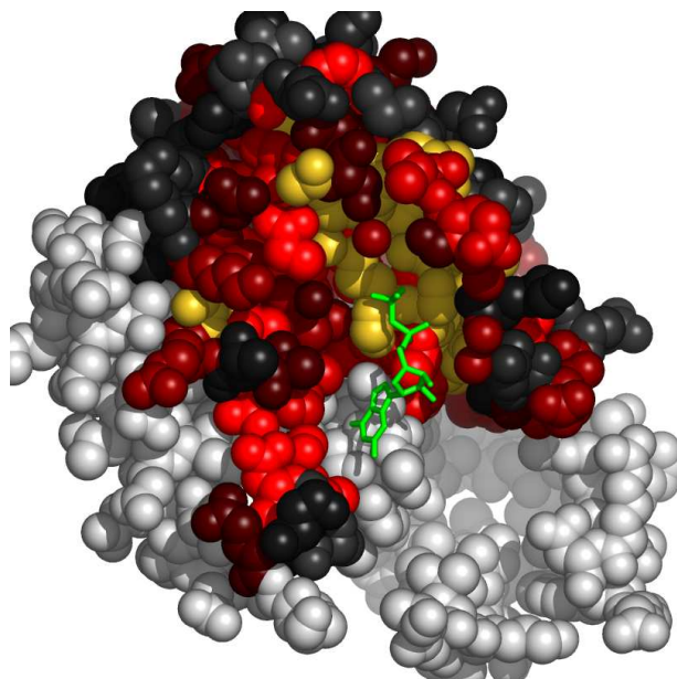
Fig. 5. Residues in 1tpzA, at the interface with GDP, colored by their relative importance. The ligand (GDP) is colored green. Atoms further than 30Å away from the geometric center of the ligand, as well as on the line of sight to the ligand were removed. (See Appendix for the coloring scheme for the protein chain 1tpzA.)
