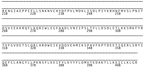
Fig. 2. Residues 218-415 in ItpzA colored by their relative importance. (See Appendix, Fig.10, for the coloring scheme.)
