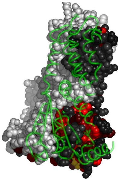
Fig. 7. Residues in ItpzA, at the interface with ItpzB, colored by their relative importance. ItpzB is shown in backbone representation (See Appendix for the coloring scheme for the protein chain ItpzA.)
