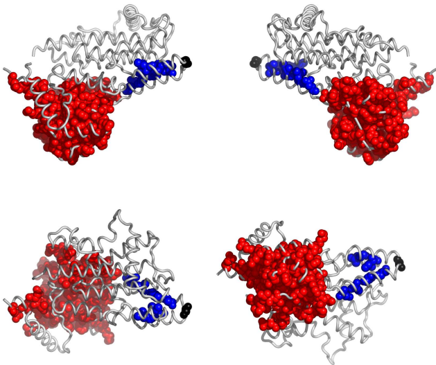
Fig. 4. Residues in ItpzA, colored according to the cluster they belong to: red, followed by blue and yellow are the largest clusters (see Appendix for the coloring scheme). Clockwise: front, back, top and bottom views. The corresponding Pymol script is attached.
