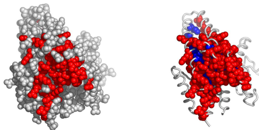
Fig. 9. A possible active surface on the chain ItpzA. The larger cluster it belongs to is shown in blue.
