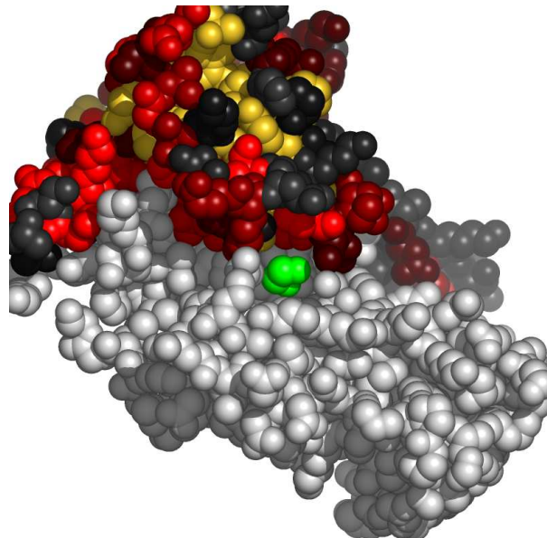
Fig. 8. Residues in ItpzA, at the interface with 1,2-ethanediol, colored by their relative importance. The ligand (1,2-ethanediol) is colored green. Atoms further than 30\text{\AA} away from the geometric center of the ligand, as well as on the line of sight to the ligand were removed. (See Appendix for the coloring scheme for the protein chain ItpzA.)
