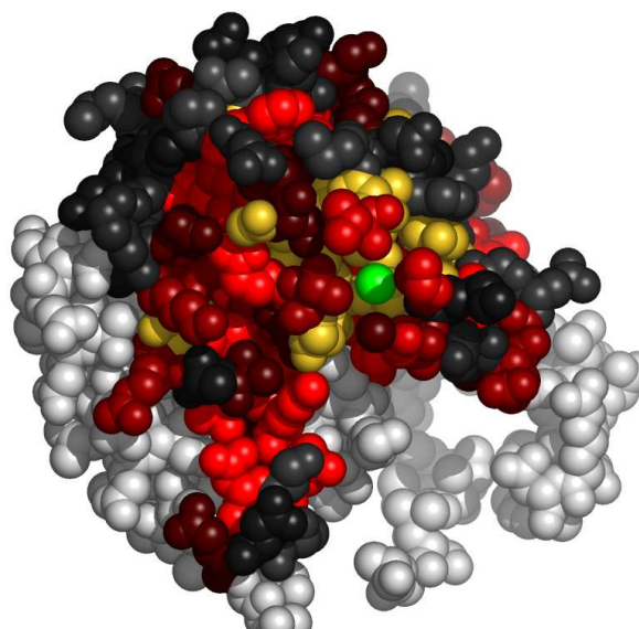
Fig. 6. Residues in 1tpzA, at the interface with magnesium ion, colored by their relative importance. The ligand (magnesium ion) is colored green. Atoms further than 30Å away from the geometric center of the ligand, as well as on the line of sight to the ligand were removed. (See Appendix for the coloring scheme for the protein chain 1tpzA.)
