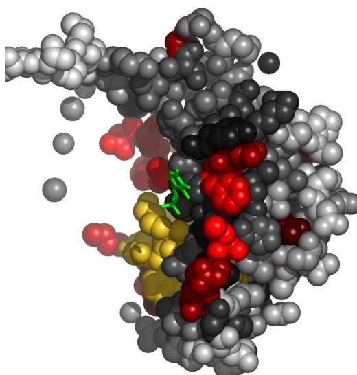
Fig. 7. Residues in 1u08A, at the interface with PLP, colored by their relative importance. The ligand (PLP) is colored green. Atoms further than 30Å away from the geometric center of the ligand, as well as on the line of sight to the ligand were removed. (See Appendix for the coloring scheme for the protein chain 1u08A.)
