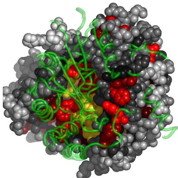
Fig. 6. Residues in 1u08A, at the interface with 1u08B, colored by their relative importance. 1u08B is shown in backbone representation (See Appendix for the coloring scheme for the protein chain 1u08A.)
