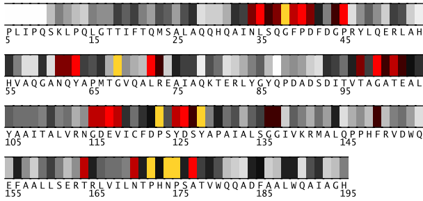
Fig. 1. Residues 5-195 in 1u08A colored by their relative importance. (See Appendix, Fig.10, for the coloring scheme.)
