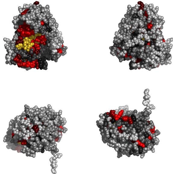
Fig. 3. Residues in 1u08A, colored by their relative importance. Clockwise: front, back, top and bottom views.
