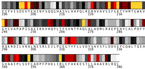
Fig. 2. Residues 196-386 in 1u08A colored by their relative importance. (See Appendix, Fig.10, for the coloring scheme.)
