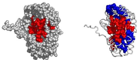
Fig. 9. Another possible active surface on the chain 1u08A. The larger cluster it belongs to is shown in blue.
