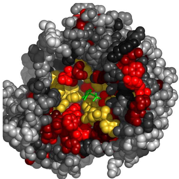
Fig. 5. Residues in 1u08A, at the interface with PLP, colored by their relative importance. The ligand (PLP) is colored green. Atoms further than 30Å away from the geometric center of the ligand, as well as on the line of sight to the ligand were removed. (See Appendix for the coloring scheme for the protein chain 1u08A.)
