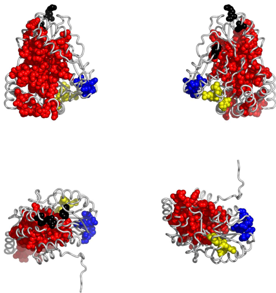
Fig. 4. Residues in 1u08A, colored according to the cluster they belong to: red, followed by blue and yellow are the largest clusters (see Appendix for the coloring scheme). Clockwise: front, back, top and bottom views. The corresponding Pymol script is attached.
